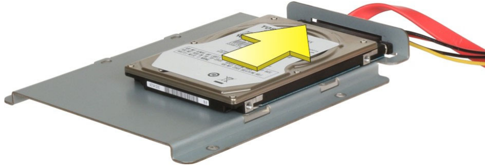
Figure 3-6: Connecting the Hard Drive to the HDD Bracket
