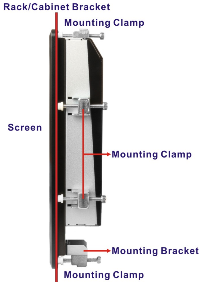
Figure 3-36: Secure the Rack/Cabinet Bracket
