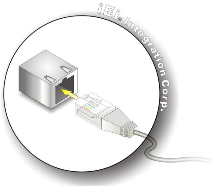
Figure 3-42: LAN Connection
