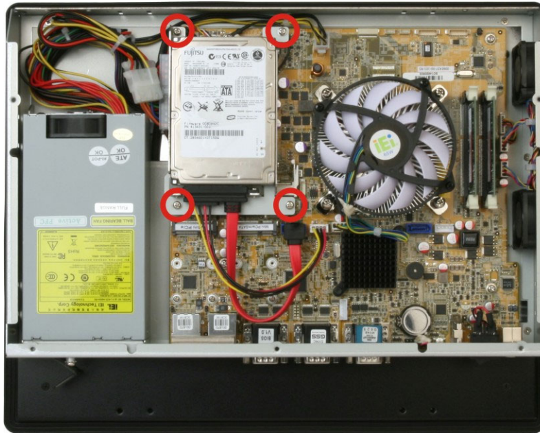
Figure 3-4: Replacing the PPC-F15A/F17A-H81 HDD Bracket
