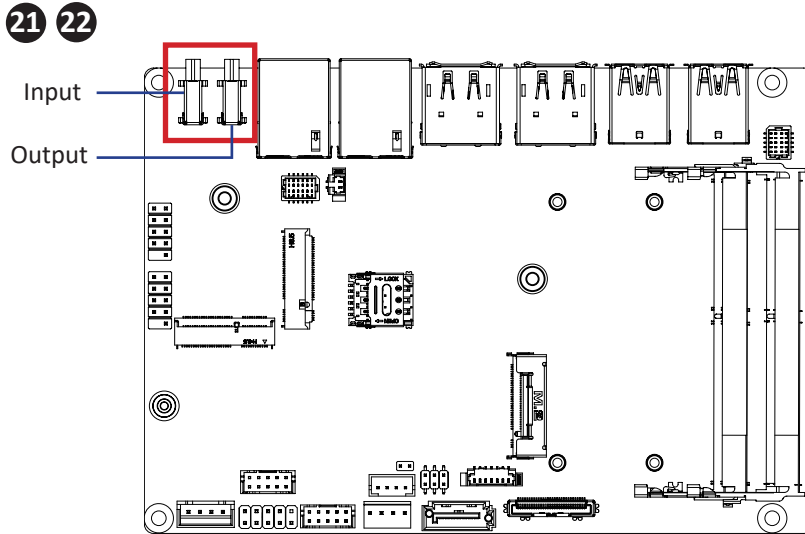
USB Type C Connector
