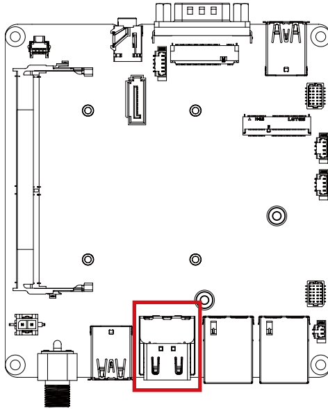
HDMI Connector
