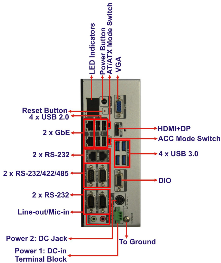
Figure 1-2: TANK-871-Q170 series Front Panel
