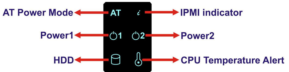
Figure 1-4: TANK-871-Q170 series LED Indicators
