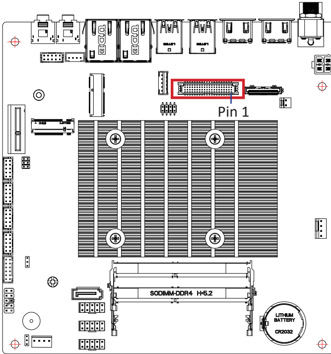
LVDS Connector
