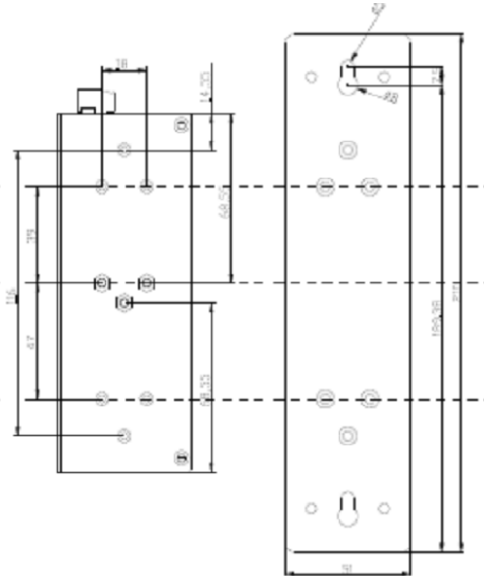
Wall-Mounting size
