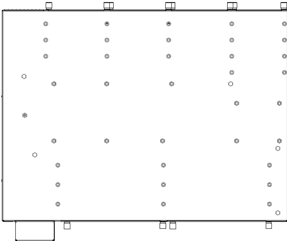
BOTTOM VIEW
