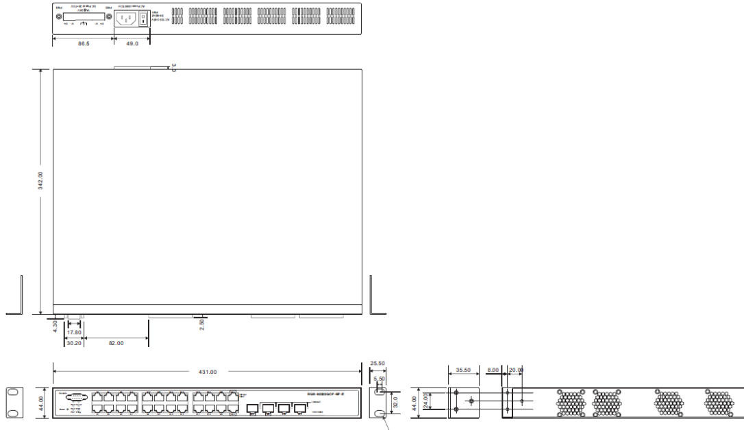
Rack-mount measurement (Unit = mm)
