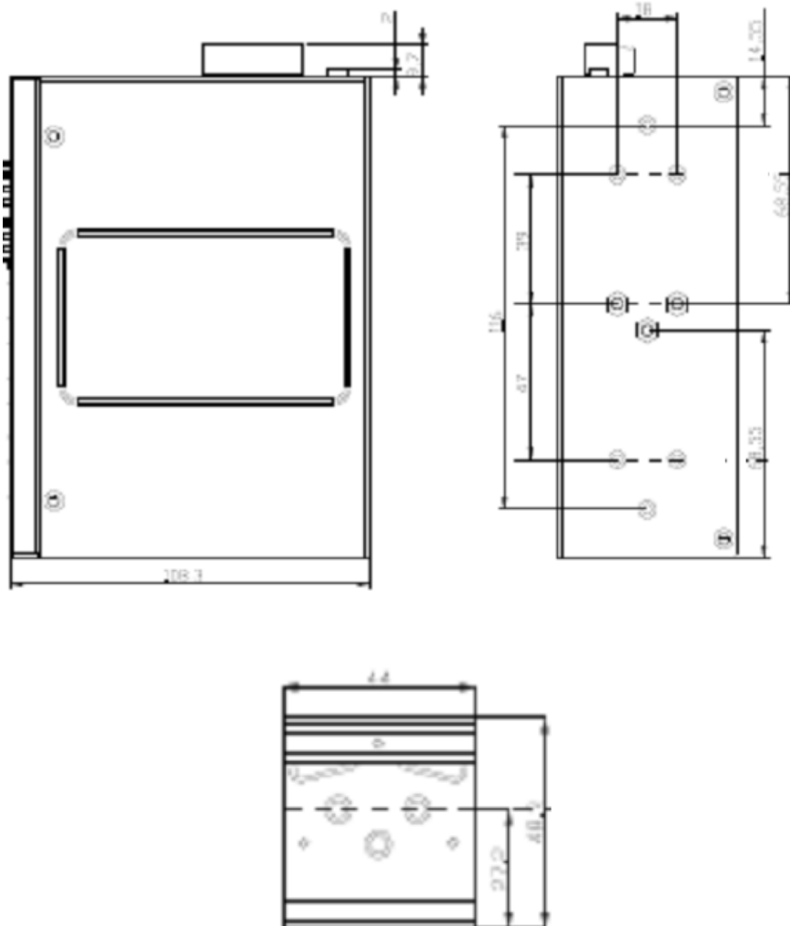
DIN-Rail Size
