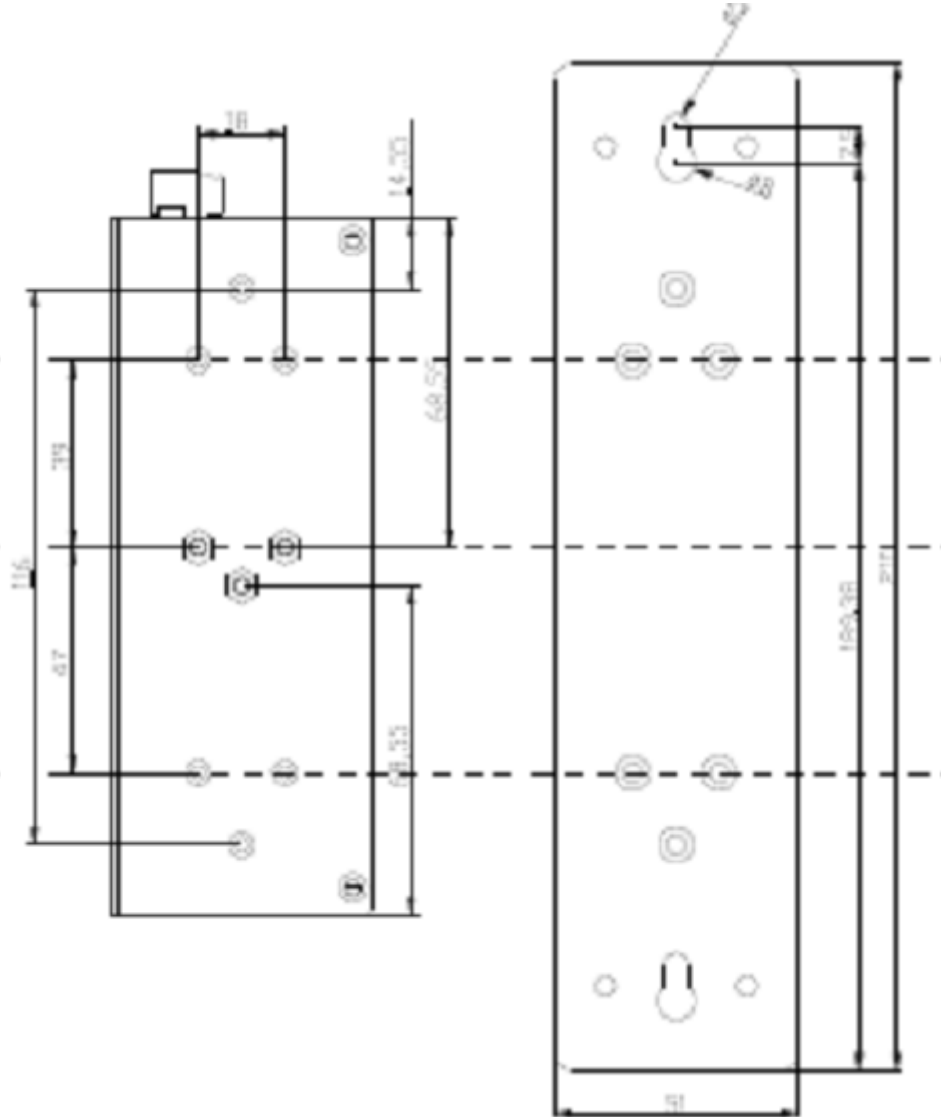
Wall-Mounting size
