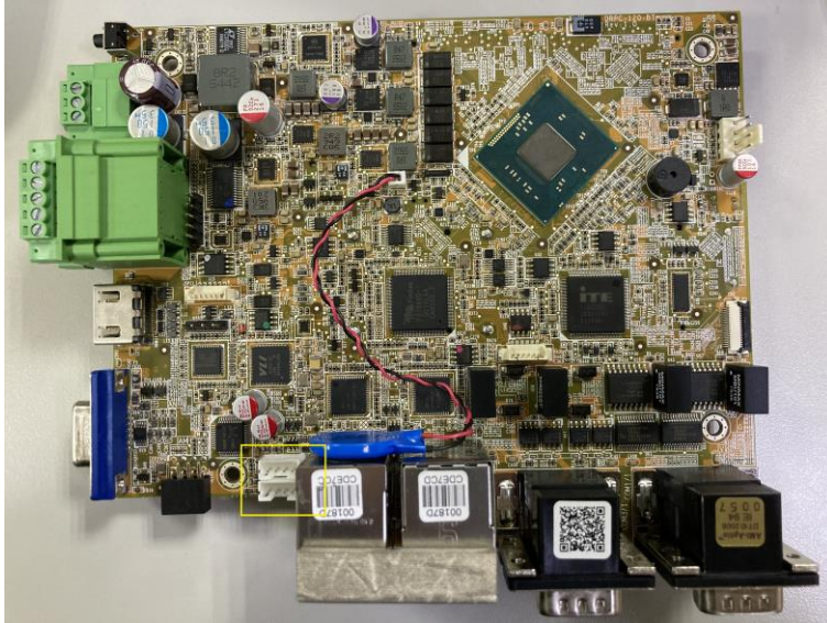
(DRPC-120-BT motherboard)
