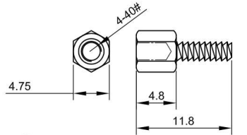
⑨ HEX SCREW 4-40#
