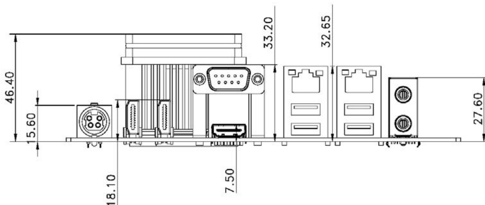
Figure 1-5: KINO-DCM236 Height Dimensions 2 (mm)
