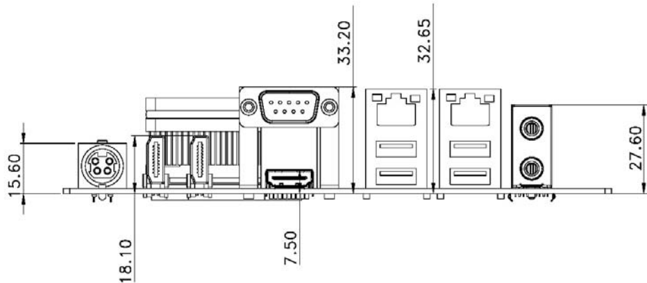
Figure 1-4: KINO-DCM236 Height Dimensions 1 (mm)
