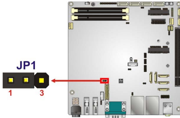
Figure 4-15: LVDS Voltage Jumper Location
