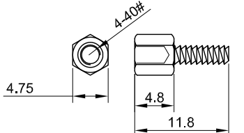
⑦ HEX SCREW 4-40#
