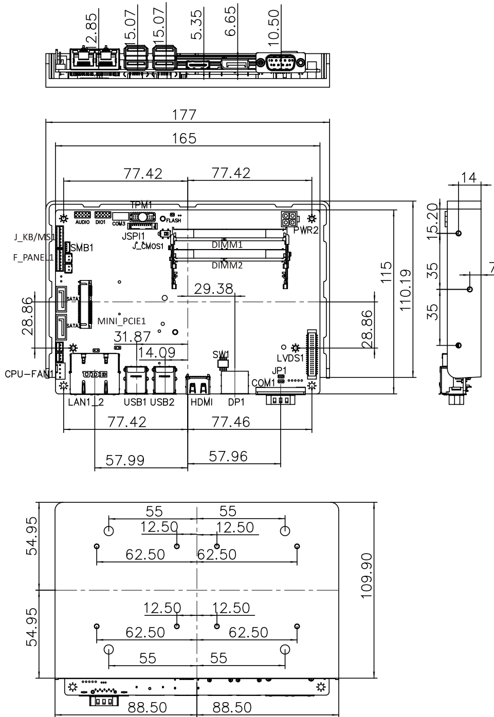
Figure 1-3: Dimensions (mm)
