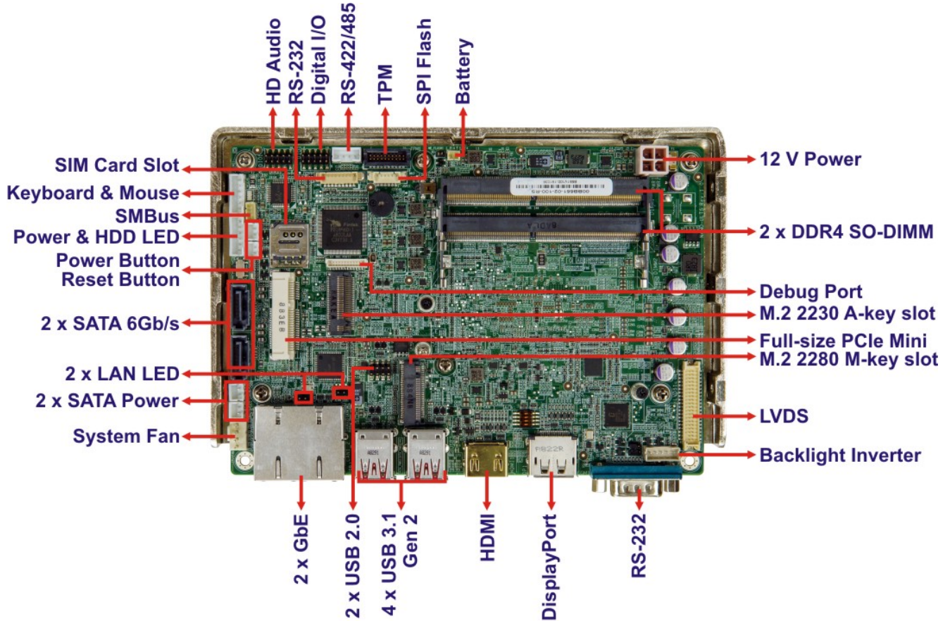
Figure 1-2: Connectors
