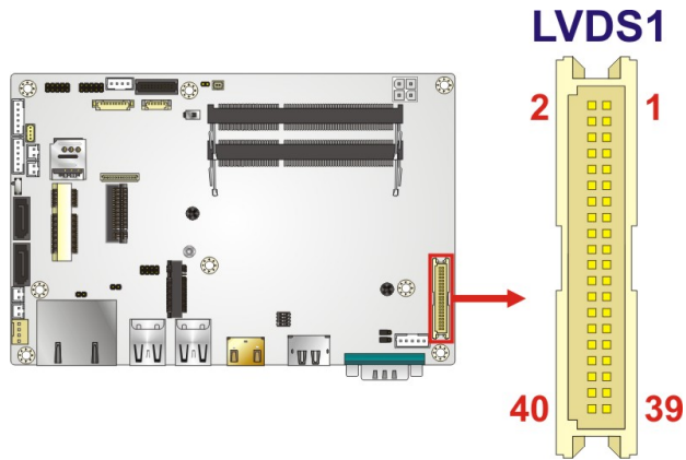
Figure 3-9: LVDS Connector Location
