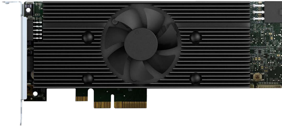
Figure 1-1: Mustang-V100-MX8
