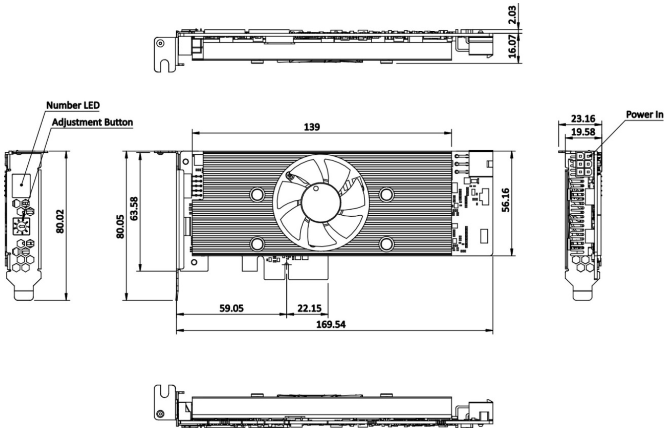
Figure 1-3: Dimensions (mm)
