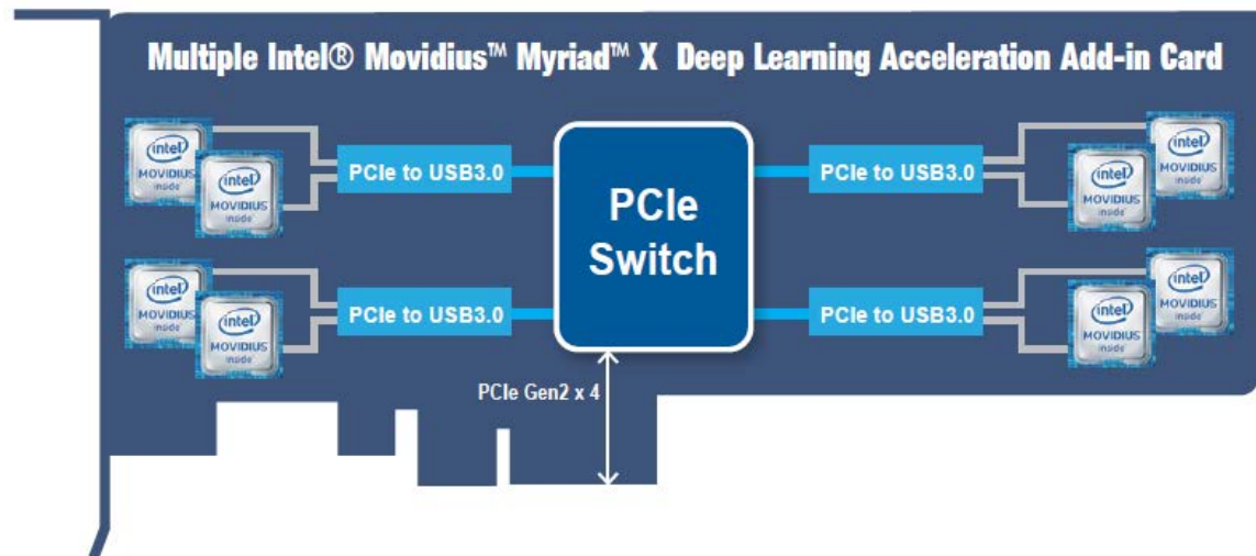
Figure 1-2: Block Diagram
