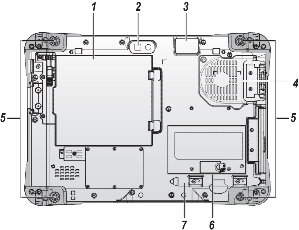
Figure 5. Rear View
