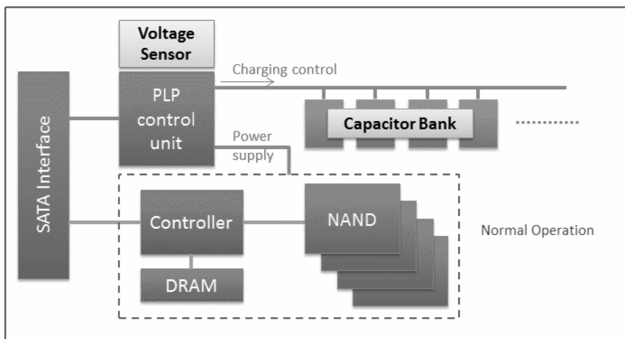
Figure 5-1 PLP architecture
