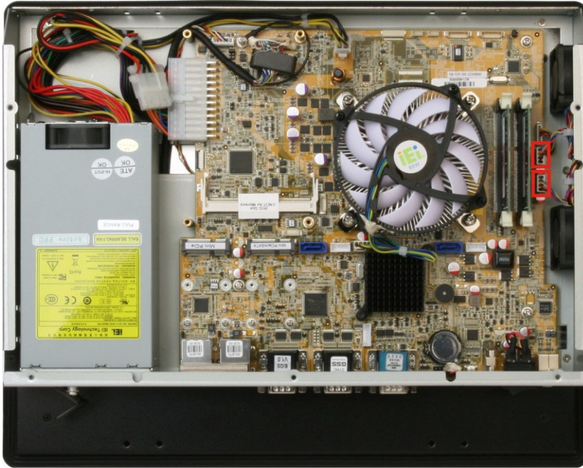
Figure 4-3: System Cooling Fans Motherboard Connectors
