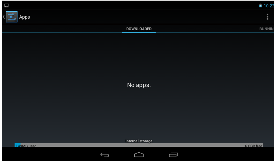
Figure 4-17: Apps Menu
