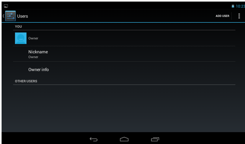
Figure 4-18: Users Menu
