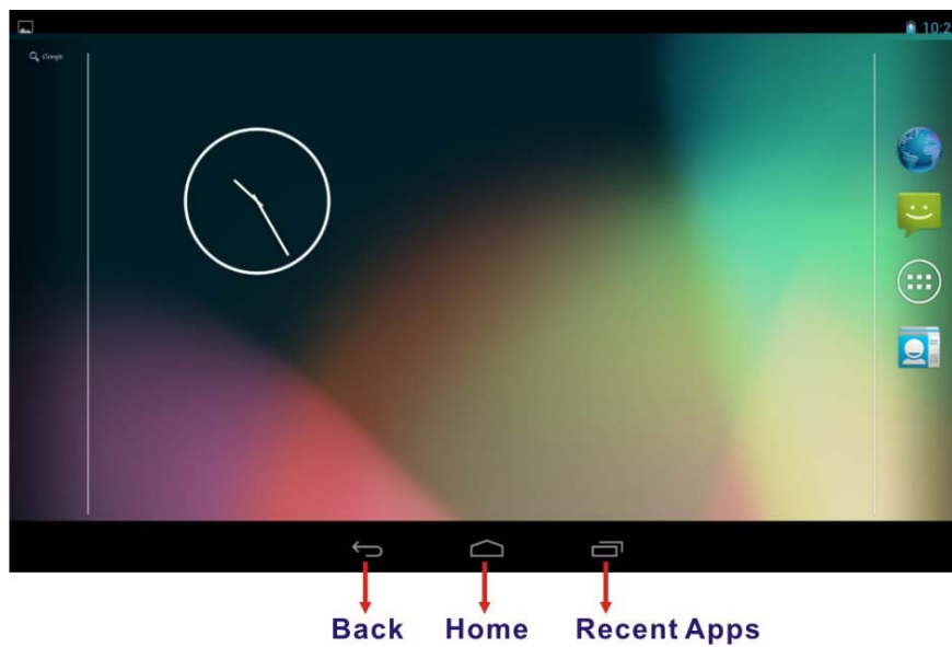
Figure 4-3: Navigation Buttons
