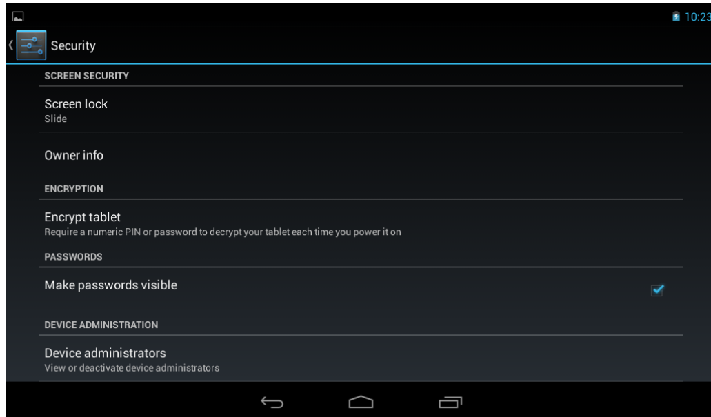
Figure 4-20: Security Menu
