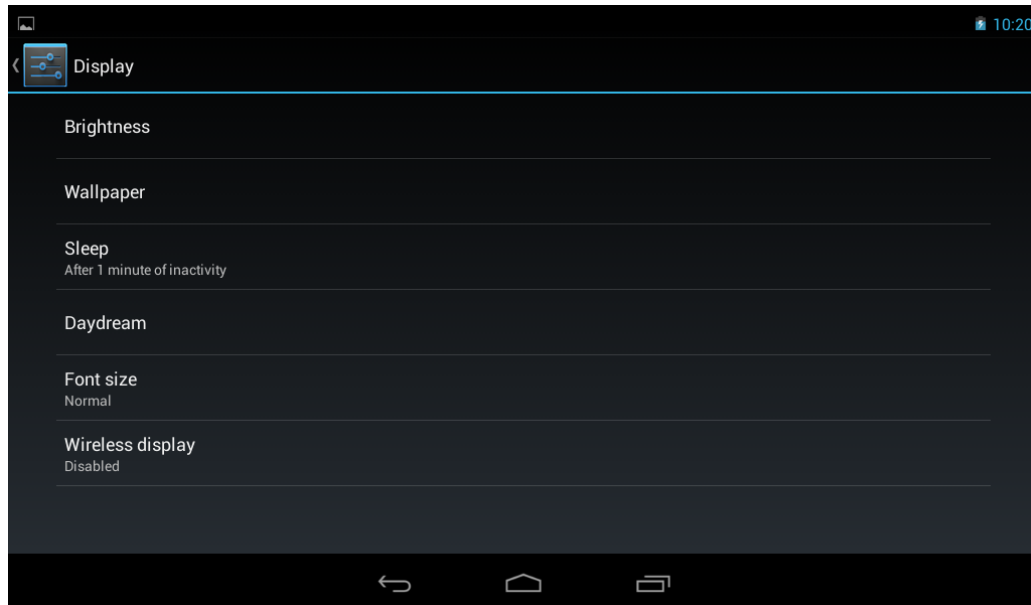
Figure 4-15: Display Menu
