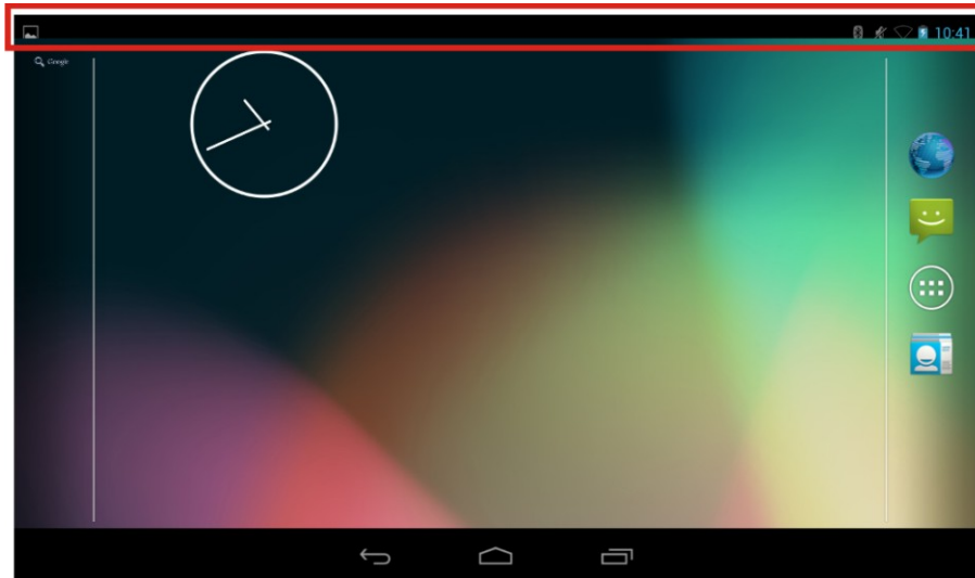
Figure 4-9: Status Bar
