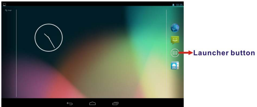
Figure 4-5: Launcher Button
