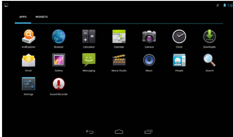
Figure 4-6: Launcher Page
