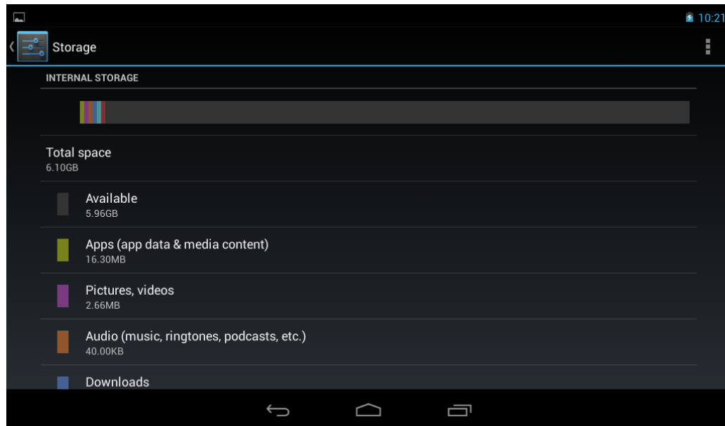
Figure 4-16: Storage Menu
