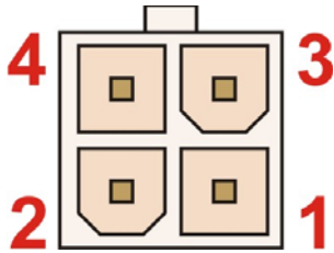
Figure 3-9: Power Input Connector
