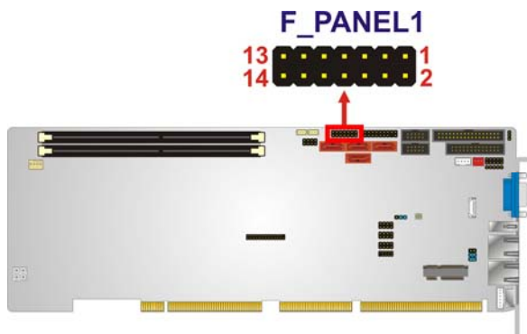
Figure 3-12: Front Panel Connector Location
