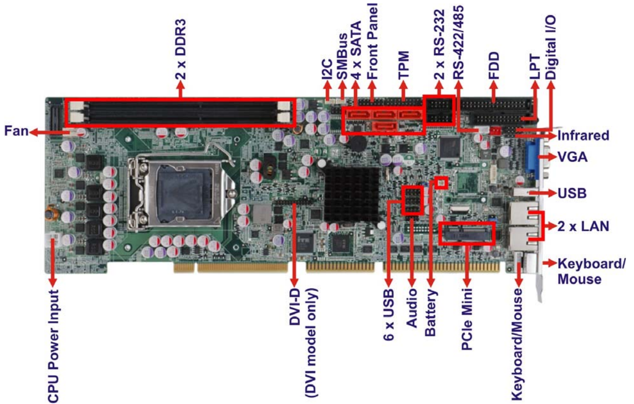
Figure 1-2: Connectors
