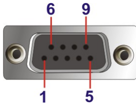
Figure 3-18: DIO Connector Pinout Location
