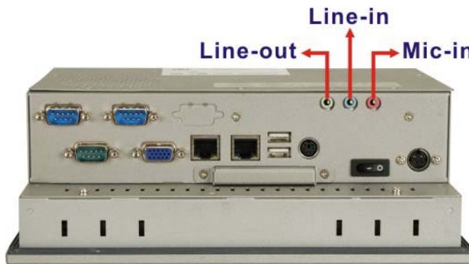
Figure 2-12: PPC-3708A Audio Jack
