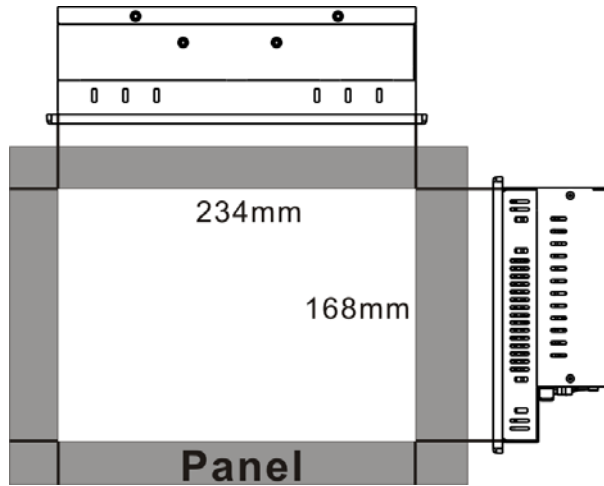
Figure 4-22: Suggested Panel Cut Out Size for PPC-3708A-N270
