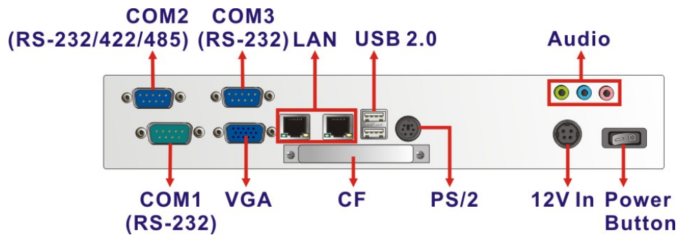
Figure 1-5: PPC-3710A-N270 Bottom View
