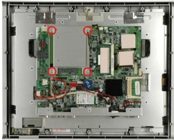
Figure 4-3: HDD Bracket Retention Screws
