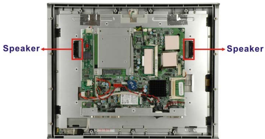
Figure 2-9: Stereo Speakers
