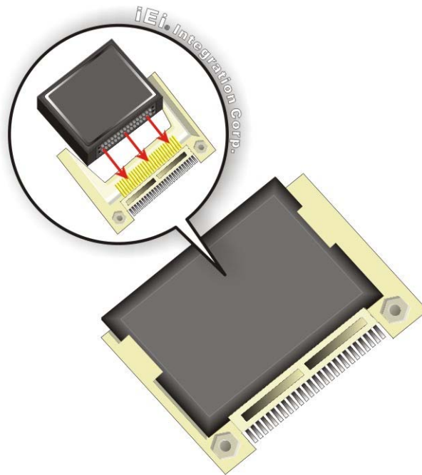
Figure 4-1: CompactFlash® Card Installation
