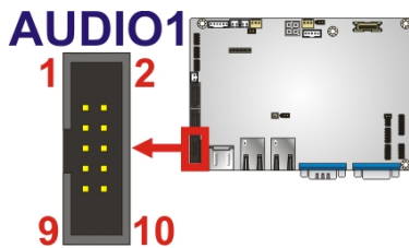
Figure 3-3: Audio Connector Location
