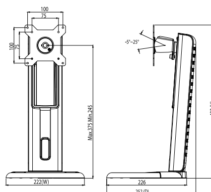
Forward/Backward Tilt (+25°/-5°)
