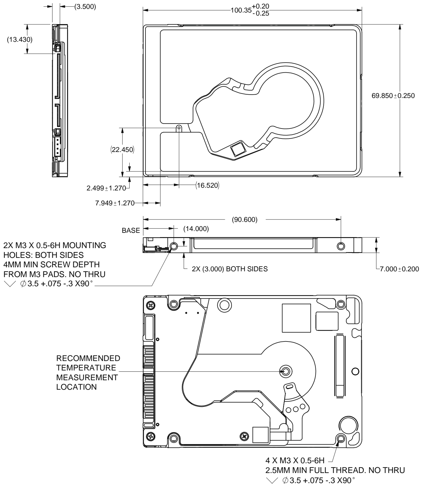
Figure 6 Mounting Dimensions (for 2-disk models)
