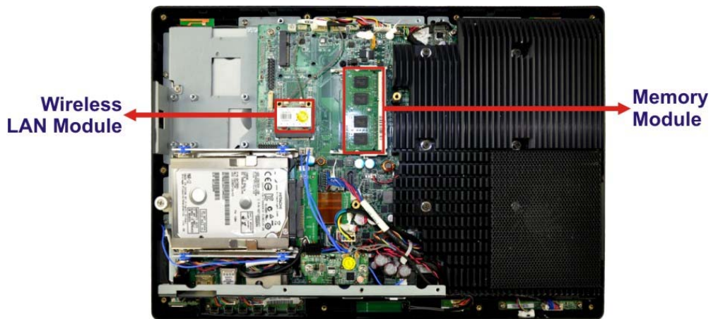
Figure 7-3: Internal Components
