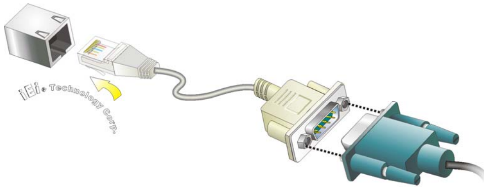
Figure 3-29: RJ-45 Serial Port Connector
