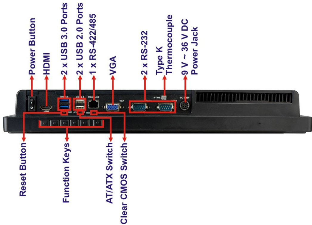
Figure 1-6: Bottom Panel
