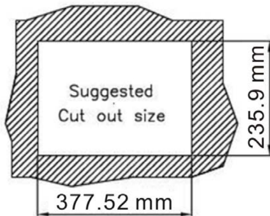
Figure 3-17: Cutout Dimensions
