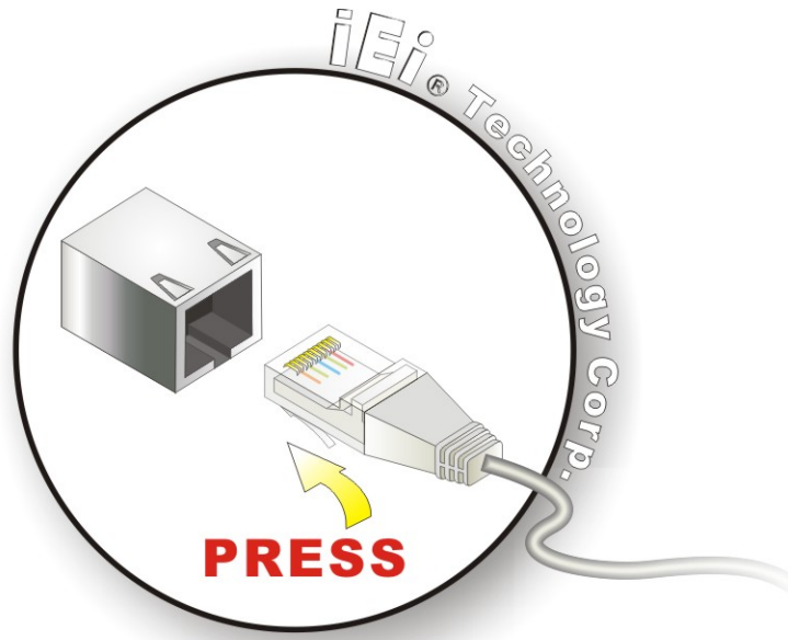
Figure 3-27: LAN Connection
