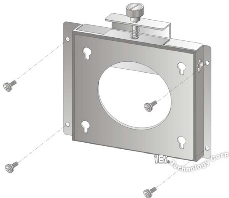
Figure 3-14: Wall-mounting Bracket
