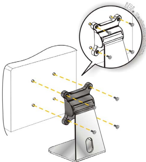
Figure 3-24: Stand Mounting (Stand-A/Bxx)
