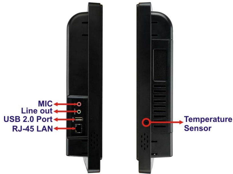
Figure 1-7: Side Panels
