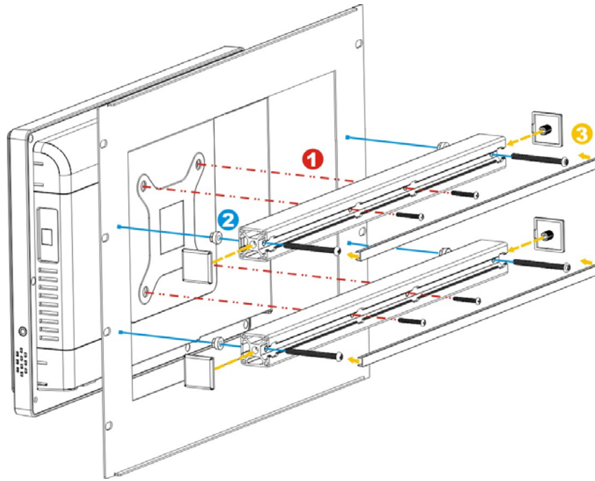
Figure 3-20: Secure the Rack/Cabinet Bracket
