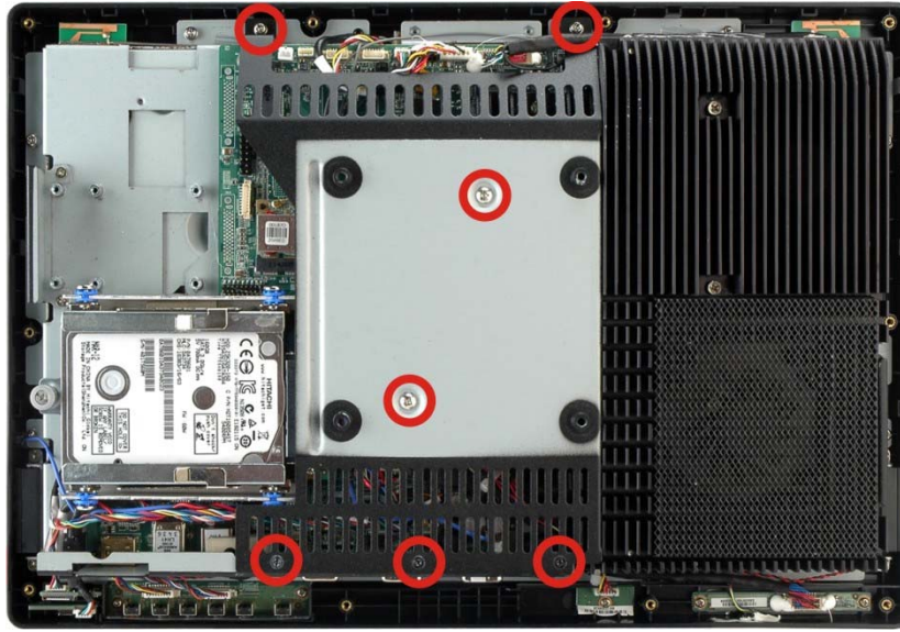
Figure 7-2: Internal Cover Retention Screws
