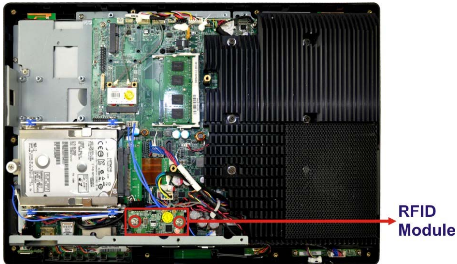
Figure 3-9: RFID Reader Module Installation
