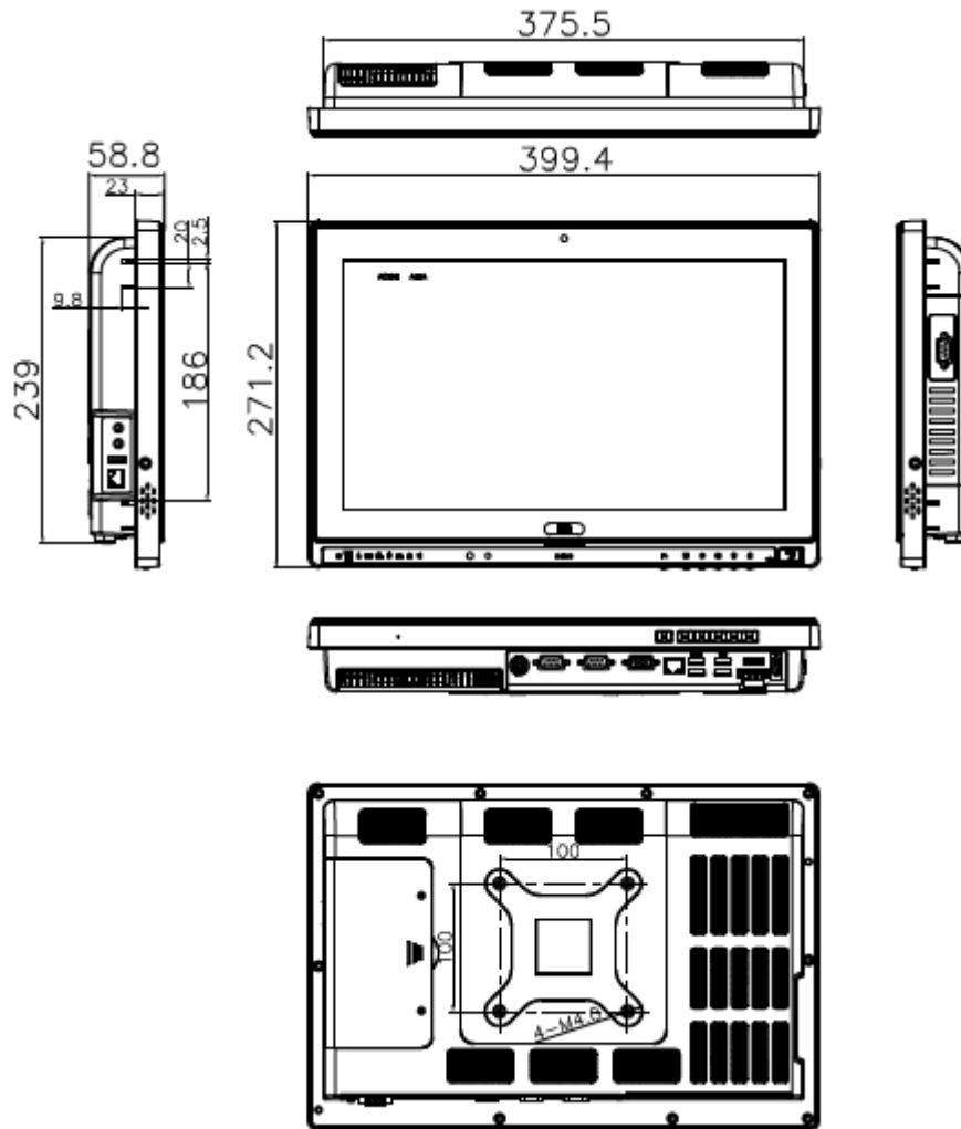
Figure 1-8: AFL2-W15B-H61 Dimensions (mm)
