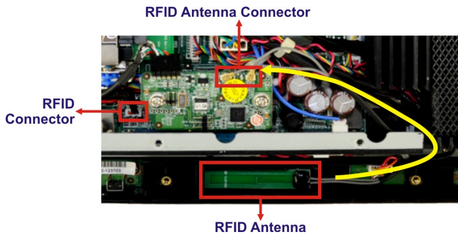
Figure 3-10: RFID Reader Connection
