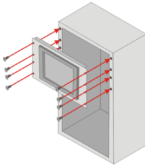
Figure 3-21: Install into a Rack/Cabinet
