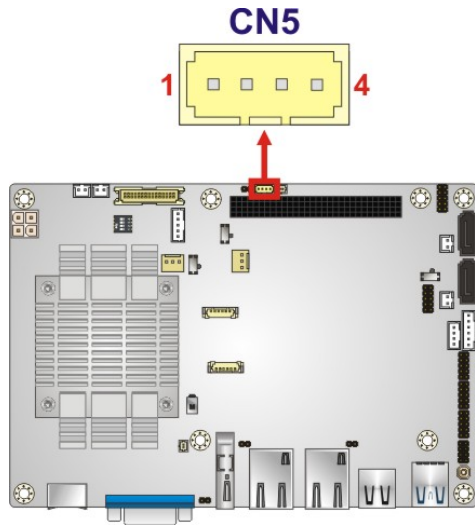
Figure 3-27: SMBus Connector Location
