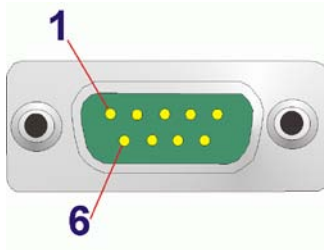
Figure 3-31: DB-9 Connector Pinout Location
