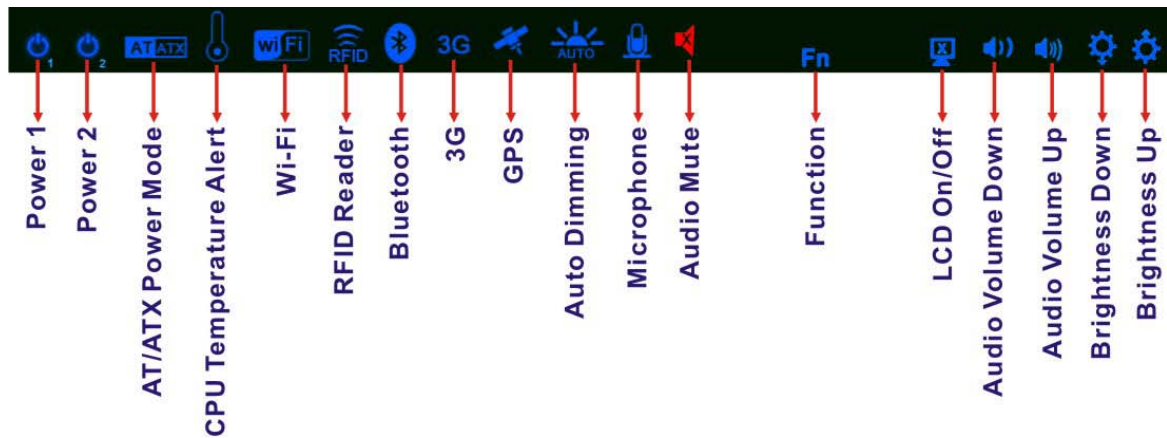
Figure 1-3: LED Indicators
