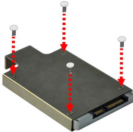
Figure 3-3: Securing the SSD
