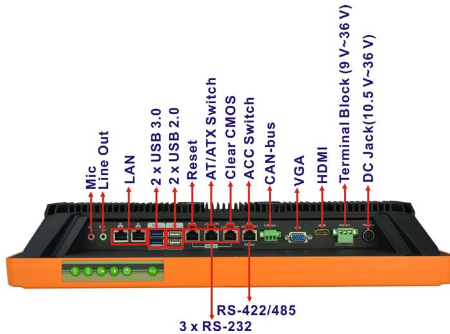
Figure 1-4: Bottom View
