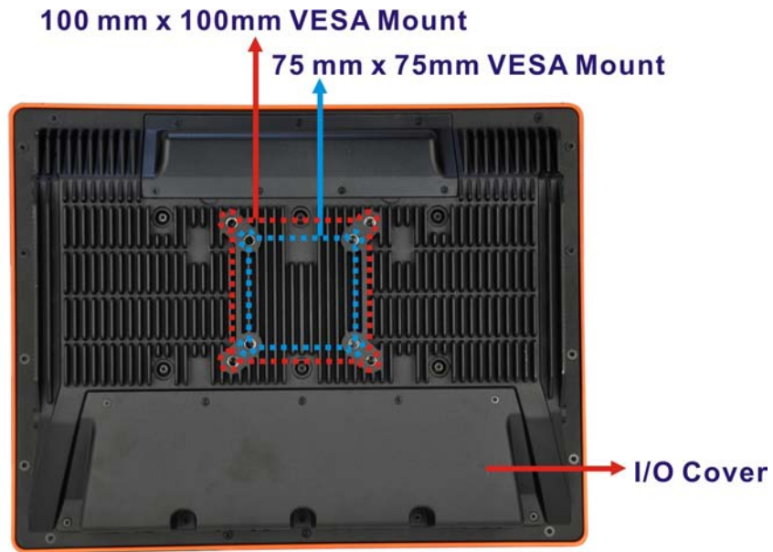
Figure 1-7: Rear View
