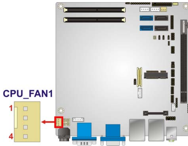
Figure 3-7: CPU Fan Connector Location
