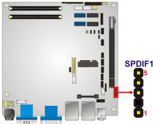
Figure 3-20: SPDIF Connector Location
