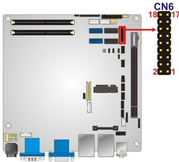
Figure 3-6: BIOS Debug Port Location
