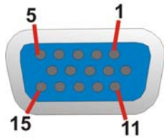
Figure 3-29: VGA Connector
