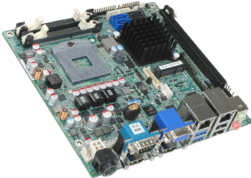
Figure 1-1: KINO-QM670
