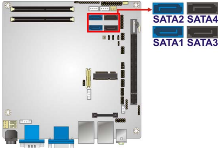
Figure 3-15: SATA Drive Connector Location
