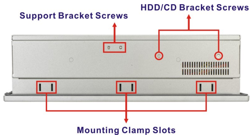
Figure 1-4: Top View
