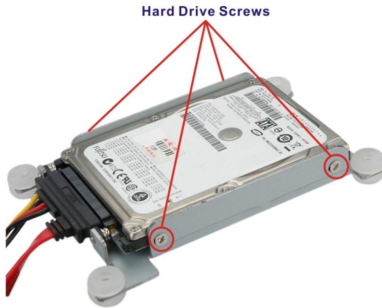
Figure 3-5: HDD Retention Screws
