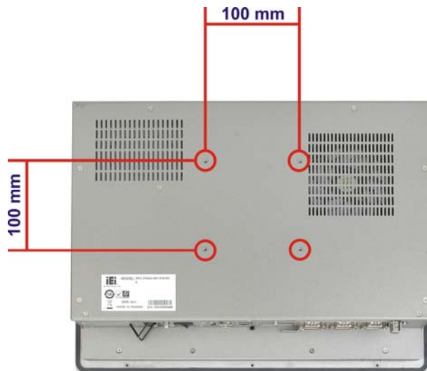
Figure 3-31: Stand Mounting Retention Screw Holes
