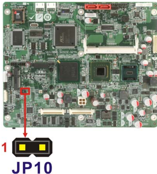
Figure 3-6: AT/ATX Power Selection Jumper Location
