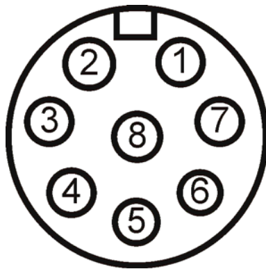
Figure 3-12: Serial Port
