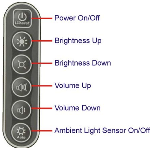
Figure 4-1: OSD Buttons
