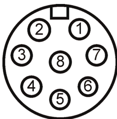
Figure 3-11: LAN Port
