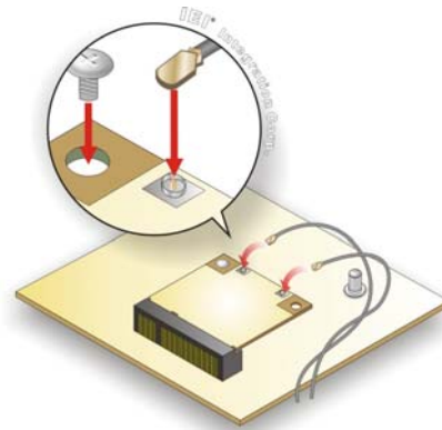
Figure 9: Removing the Retention Screw
