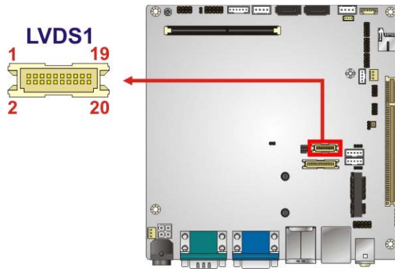
Figure 3-8: LVDS1 Connector Location
