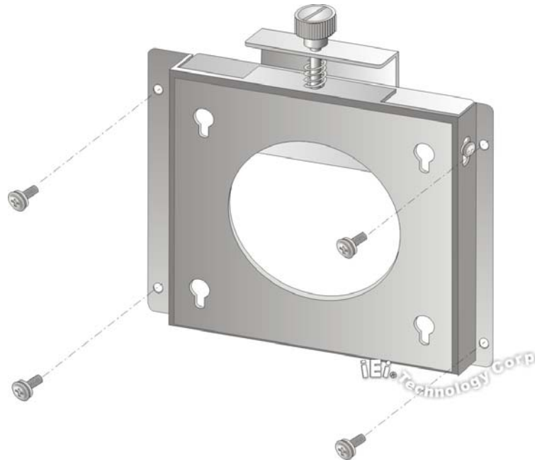
Figure 4-10: Wall-mounting Bracket
