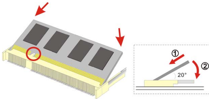
Figure 5-3: DDR SO-DIMM Module Installation
