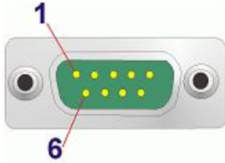
Figure 4-19: DB-9 Connector
