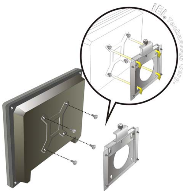
Figure 4-11: Chassis Support Screws
