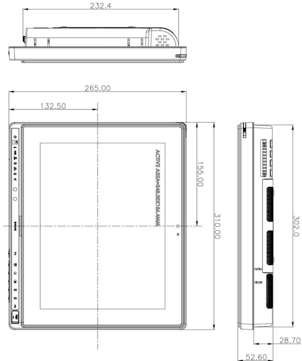
Figure 2-1: AFL2-12A-D525 Dimensions (mm)
