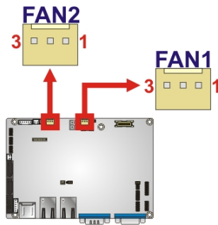
Figure 3-6: Fan Connector Locations
