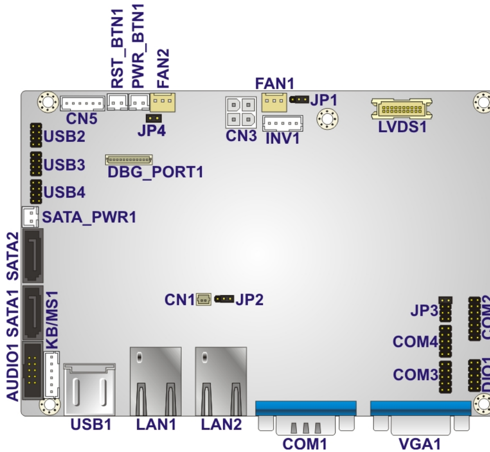
Figure 3-1: Connector and Jumper Locations (Front Side)
