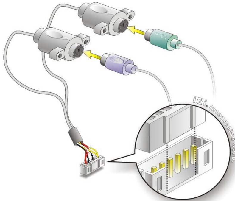
Figure 4-9: Keyboard/mouse Y-cable Connection
