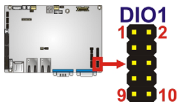
Figure 3-5: Digital I/O Connector Location
