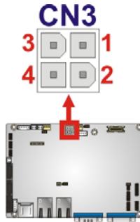
Figure 3-14: LED and +5 V Power Output Connector Location
