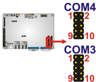
Figure 3-16: RS-232 Serial Port Connector Location
