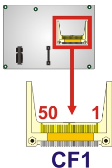
Figure 3-4: CompactFlash® Slot Location
