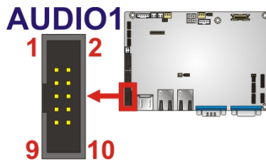
Figure 3-3: Audio Connector Location
