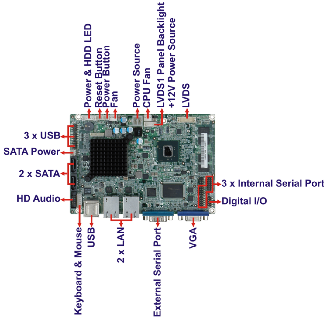
Figure 1-2: Connectors (Top side)
