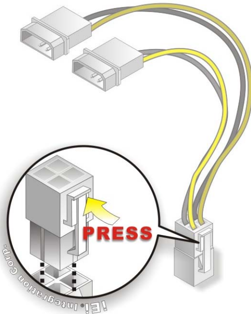
Figure 4-6: Power Cable to Motherboard Connection
