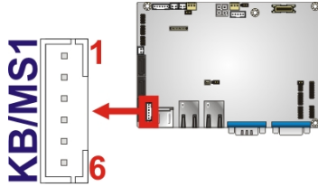
Figure 3-7: Keyboard/Mouse Connector Location
