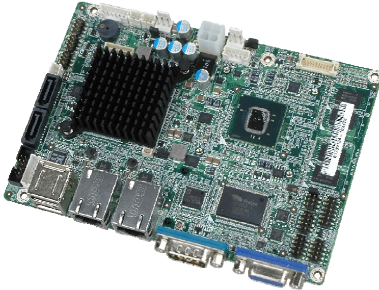
Figure 1-1: WAFER-PV-D4251/D5251/N4551
