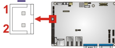
Figure 3-18: SATA Power Connector Locations
