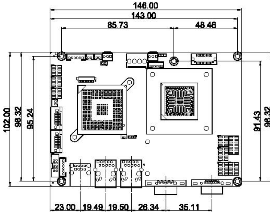
Figure 1-4: Dimensions without Heatsink (mm)
