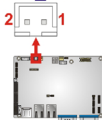
Figure 3-11: Power Button Connector Location
