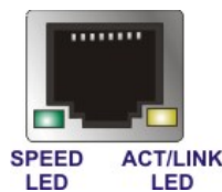
Figure 3-21: Ethernet Connector
