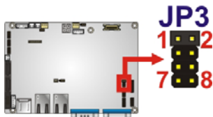
Figure 4-4: COM2 Port Mode Setting Jumper Location
