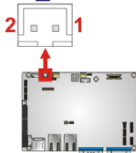
Figure 3-12: Reset Button Connector Location
