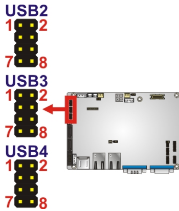
Figure 3-19: USB Connector Location
