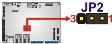
Figure 4-3: Clear CMOS Jumper Location
