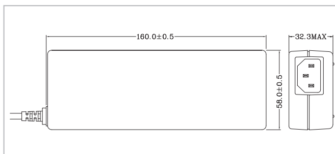
Plug Type: øin 2.5 mm / øout 5.5 mm
