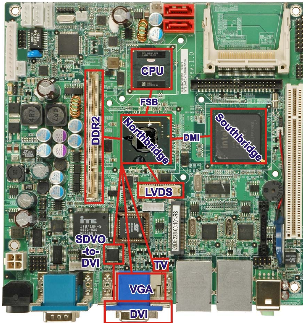
Figure 2-4: Chipset
