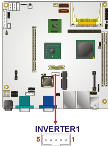
Figure 4-10: LCD Backlight Connector Pinout Locations
