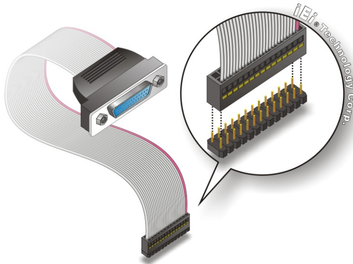
Figure 5-10: LPT Cable Connection
