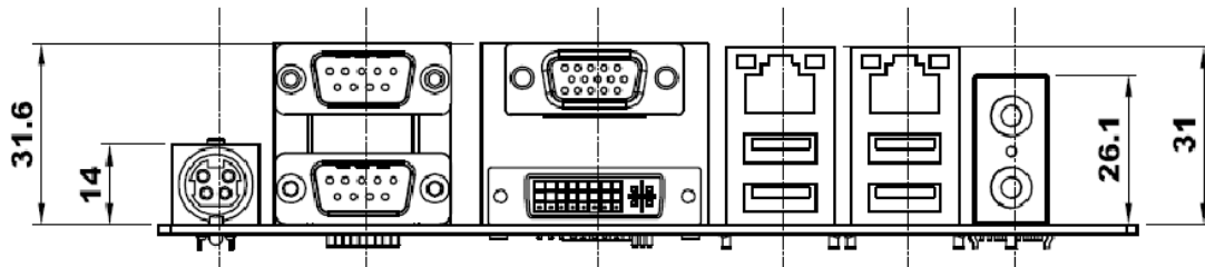
Figure 2-2: External Interface Panel Dimensions (mm)
