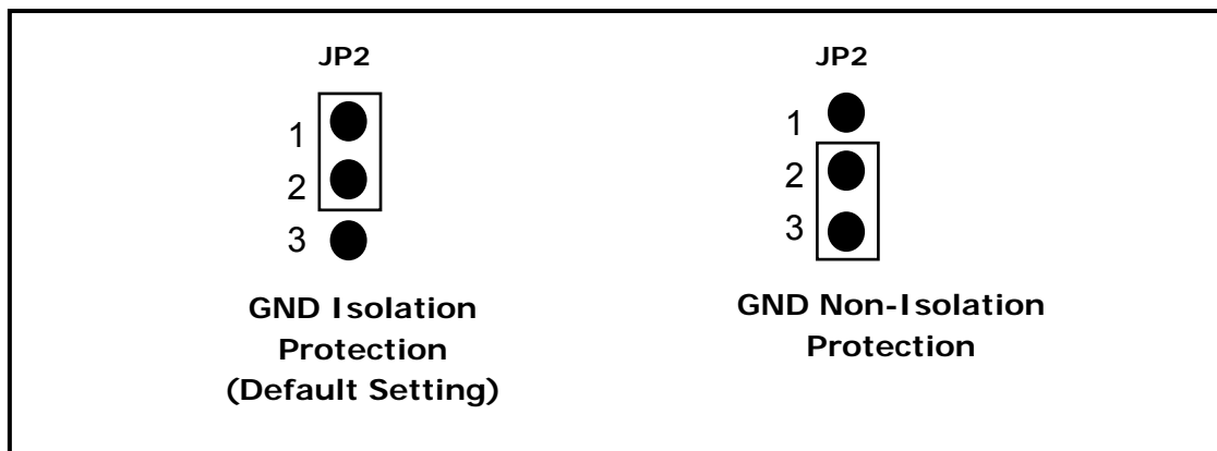
Figure 1-12: Jumper Settings
