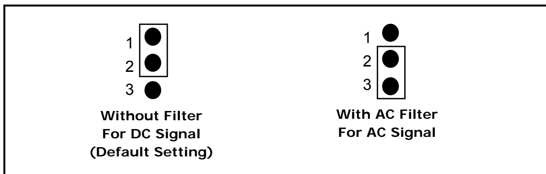
Figure 1-11: Jumper Settings
