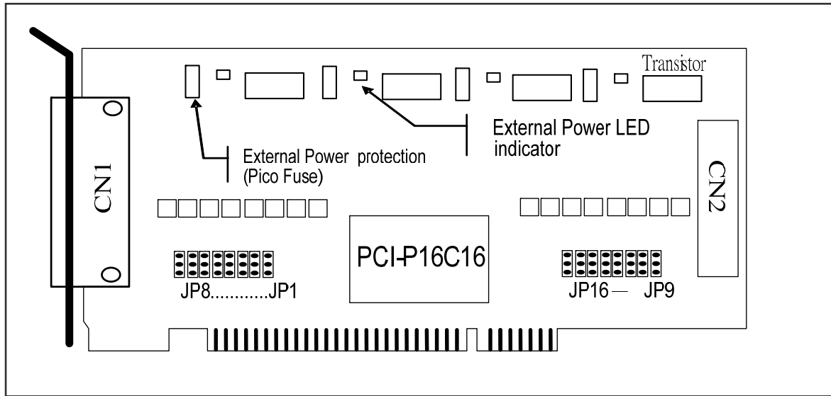
Figure 1-4: PCI -P16C16 Layout
