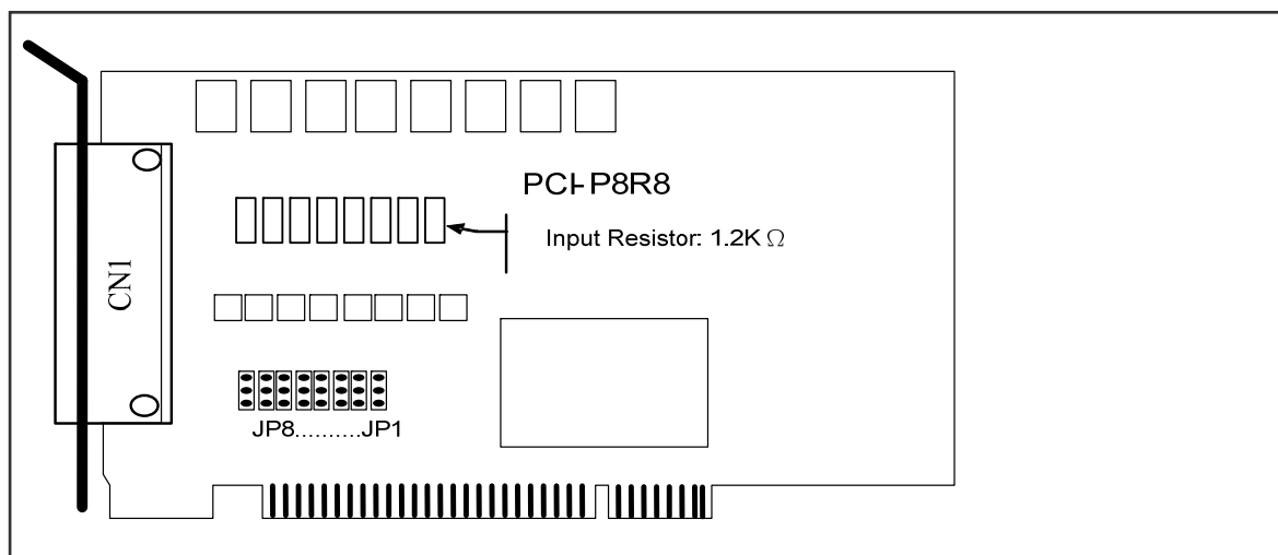
Figure 1-2: PCI-P8R8 Layout
