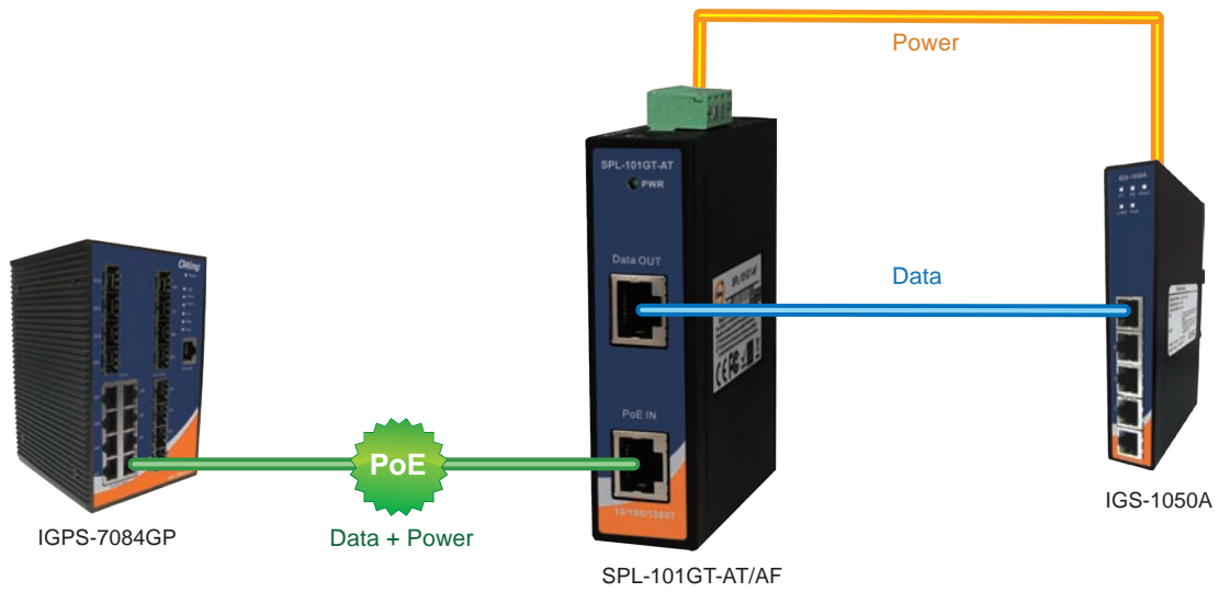
PoE Splitter Connections
