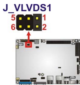
Figure 4-10: LVDS Voltage Selection Jumper Locations
