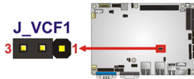
Figure 4-8: CompactFlash® Voltage Selection Jumper Location
