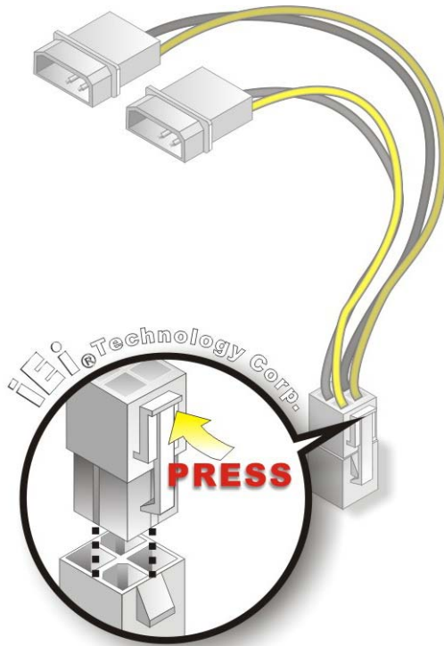
Figure 4-12: Power Cable to Motherboard Connection
