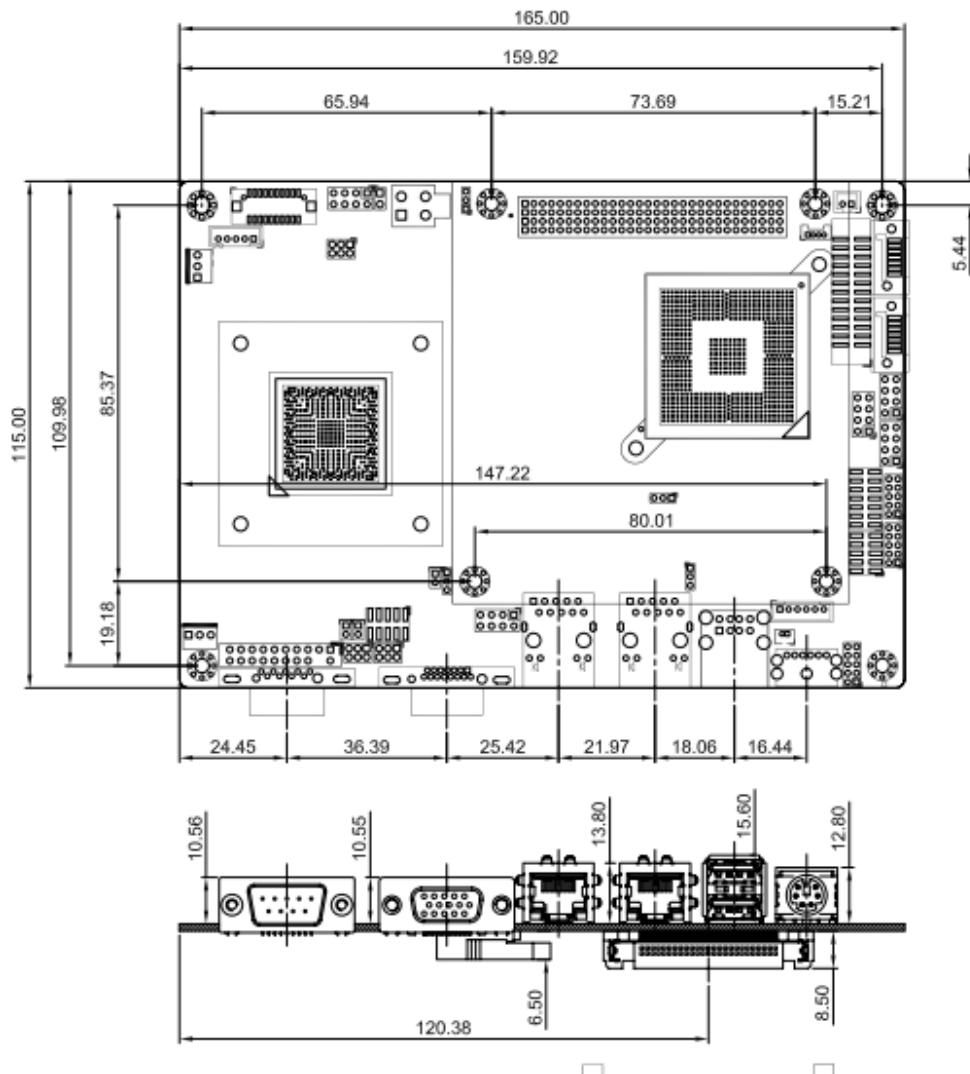
Figure 1-3: NANO-PV-D4251/N4551/D5251 Dimensions (mm)
