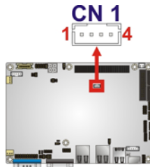
Figure 3-20: SMBus Connector Locations
