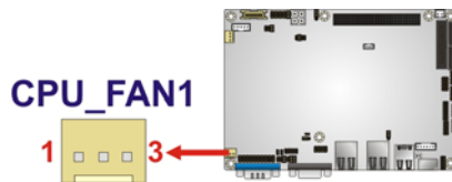
Figure 3-6: CPU Fan Connector Location
