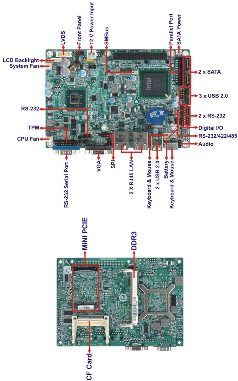
Figure 1-2: Connectors
