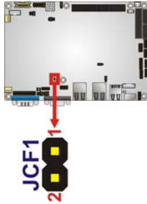
Figure 4-7: CompactFlash® Setup Jumper Location
