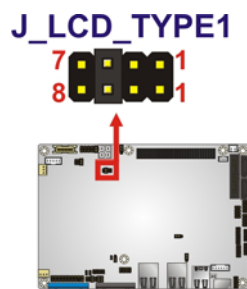
Figure 4-9: LVDS Screen Resolution Jumper Locations
