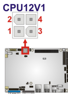
Figure 3-15: CPU 12V Power Connector Location
