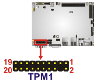
Figure 3-22: TPM Connector Pinout Locations
