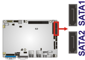
Figure 3-16: SATA Drive Connector Locations
