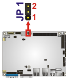
Figure 4-11: PCI-104 Voltage Jumper Location
