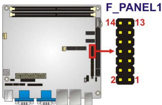
Figure 3-7: Front Panel Connector Location
