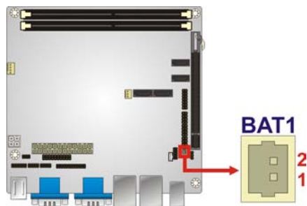
Figure 3-2: Battery Connector Location
