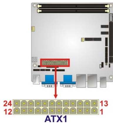
Figure 3-10: Power Connector Location
