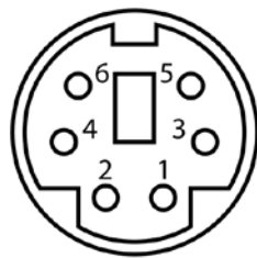
Figure 3-20: PS/2 Pinout and Configuration
