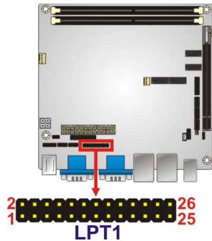
Figure 3-9: Parallel Port Connector Location
