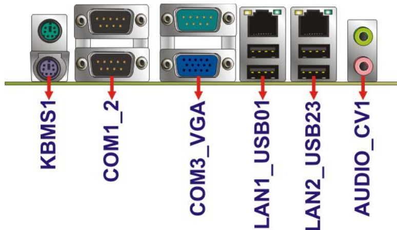
Figure 3-18: External Peripheral Interface Connector
