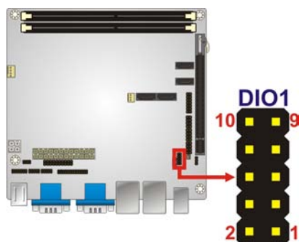
Figure 3-6: Digital I/O Connector Locations
