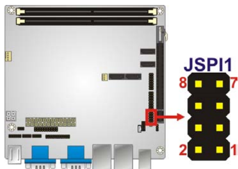
Figure 3-15: SPI Flash Connector
