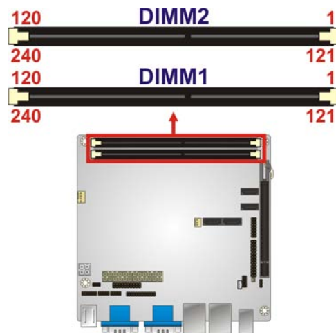
Figure 3-8: Memory Card Slot Location
