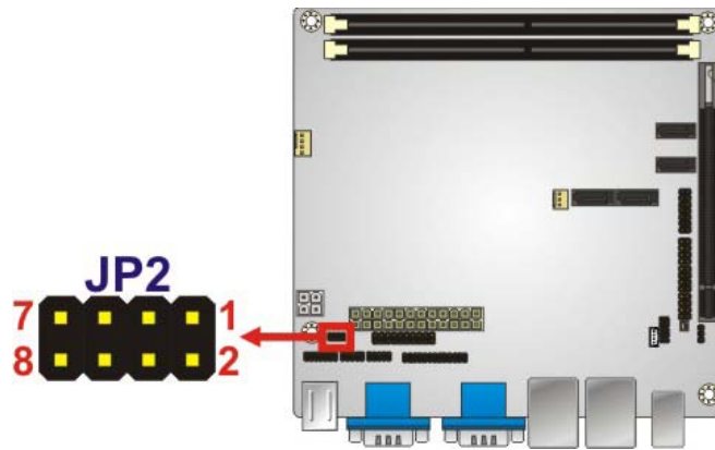
Figure 4-9: COM 6 Function Select Jumper Location
