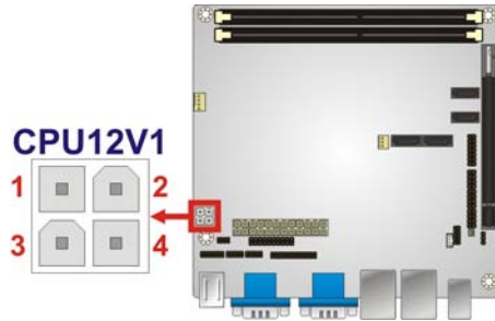
Figure 3-5: CPU Power Input Connector Location
