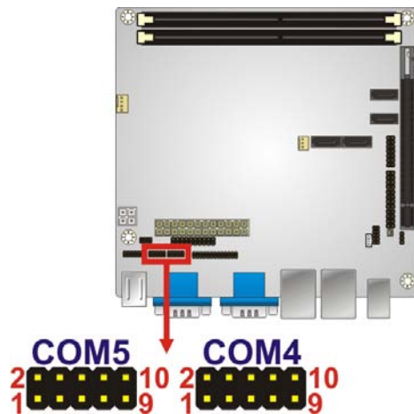
Figure 3-11: Serial Port Connector Location
