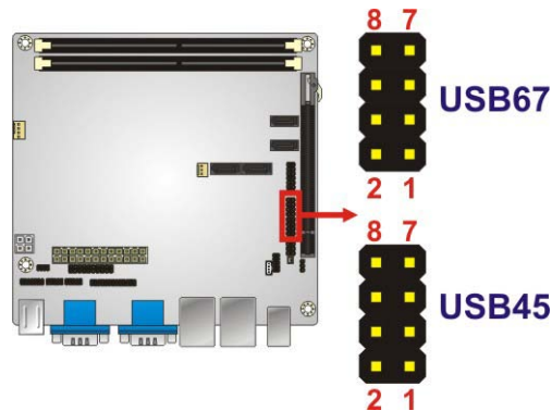
Figure 3-16: USB Connector Pinout Locations
