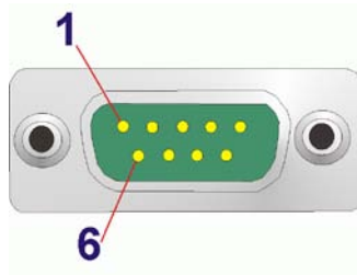
Figure 3-21: Serial Port Pinouts
