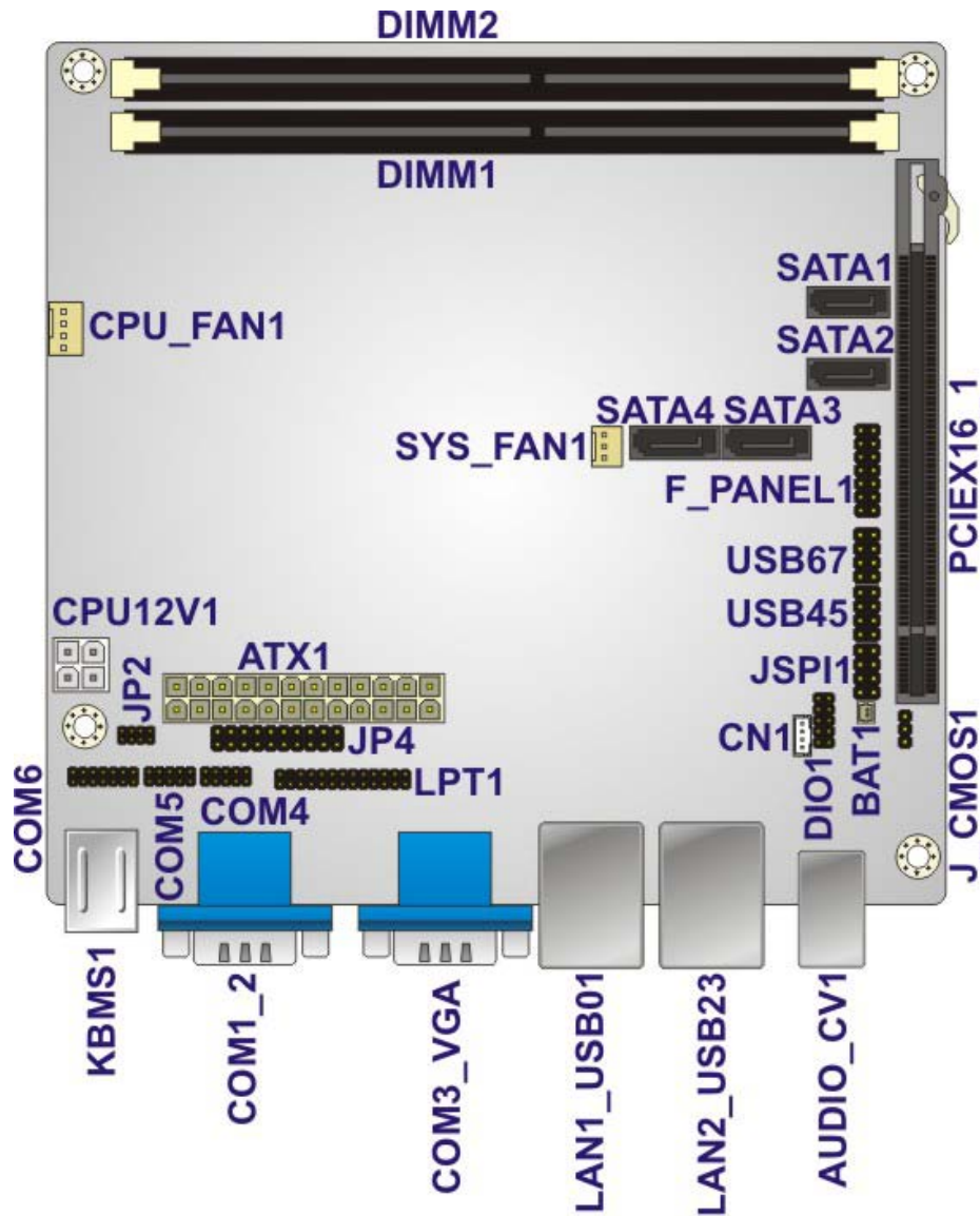
Figure 3-1: Connectors and Jumpers
