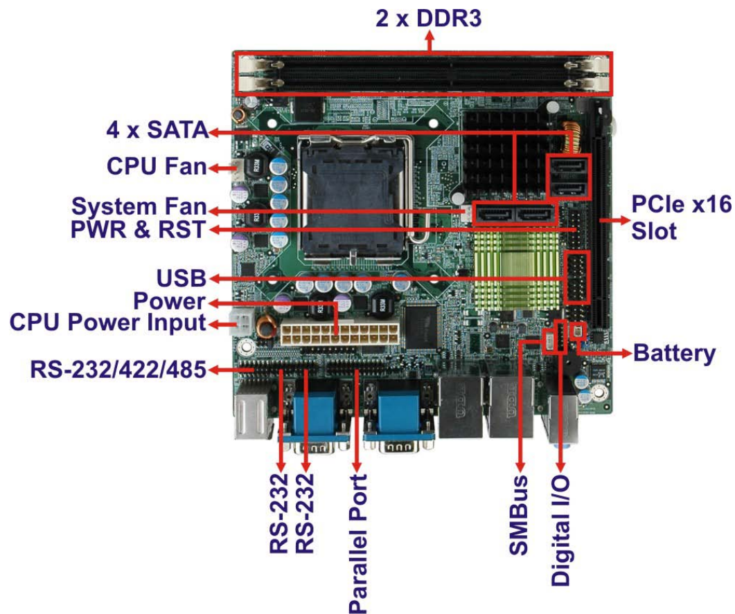
Figure 1-2: Connectors
