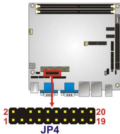
Figure 3-17: VGA to LVDS Connector Location
