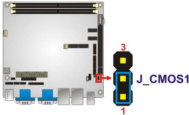
Figure 4-8: Clear BIOS Jumper Location
