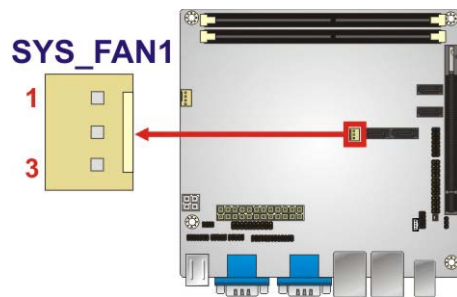
Figure 3-4: CPU Fan Connector Location
