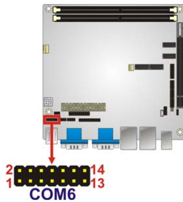
Figure 3-12: RS-232/422/485 Serial Port Connector Location
