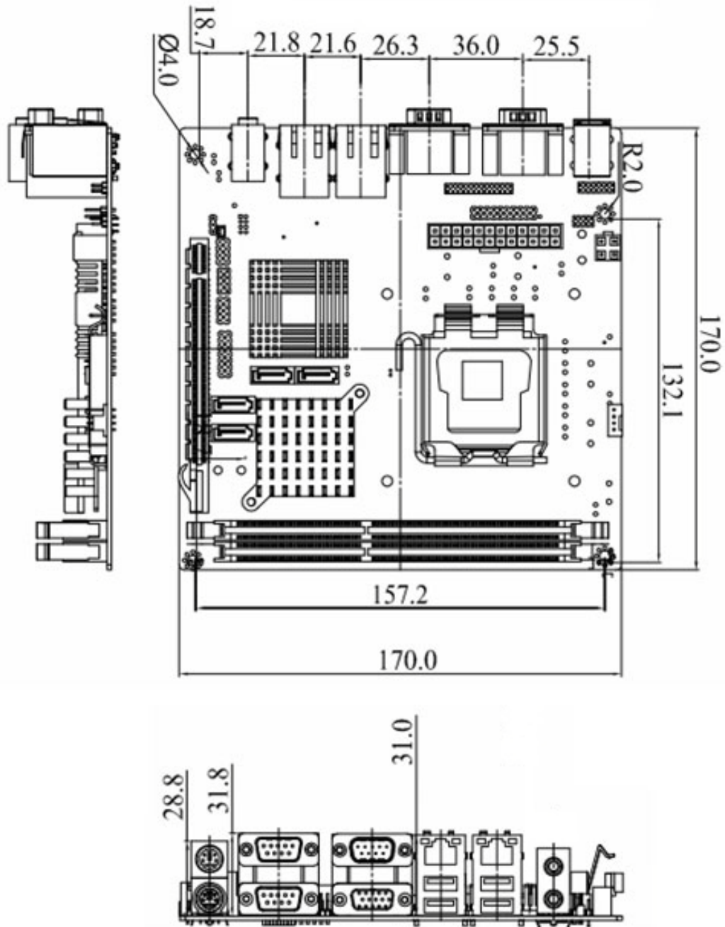
Figure 1-3: Dimensions (mm)
