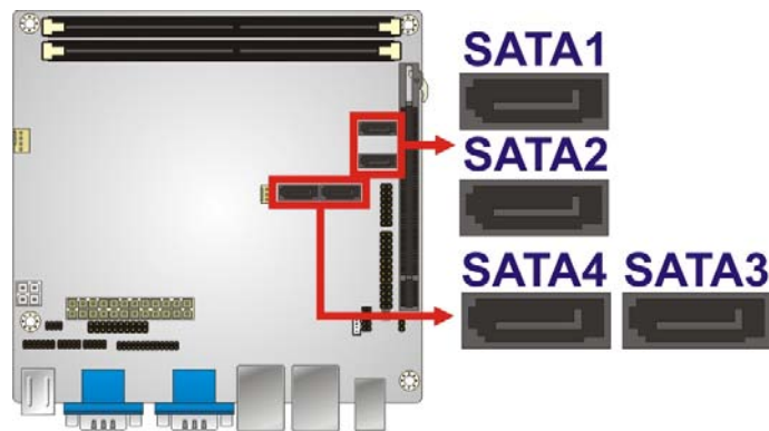
Figure 3-13: SATA Drive Connector Location
