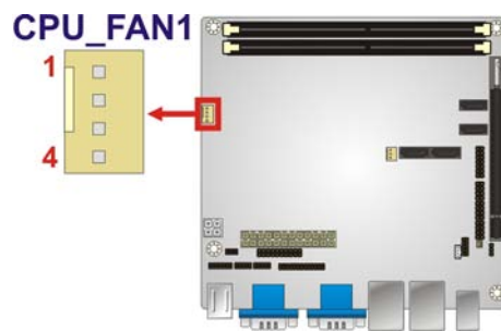
Figure 3-3: CPU Fan Connector Location
