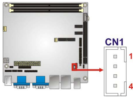
Figure 3-14: SMBus Connector Location
