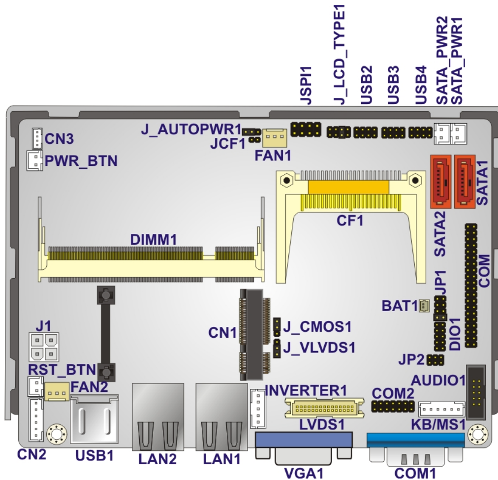
Figure 3-1: Connector and Jumper Locations
