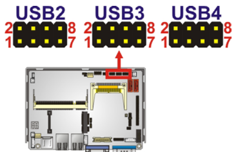
Figure 3-22: USB Connector Location
