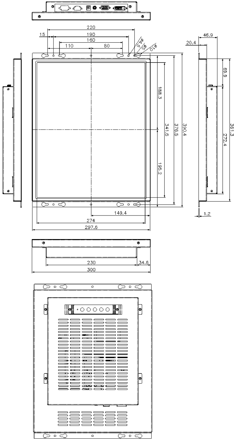
Figure 2-4: LCD-KIT170G Physical Dimensions (millimeters)
