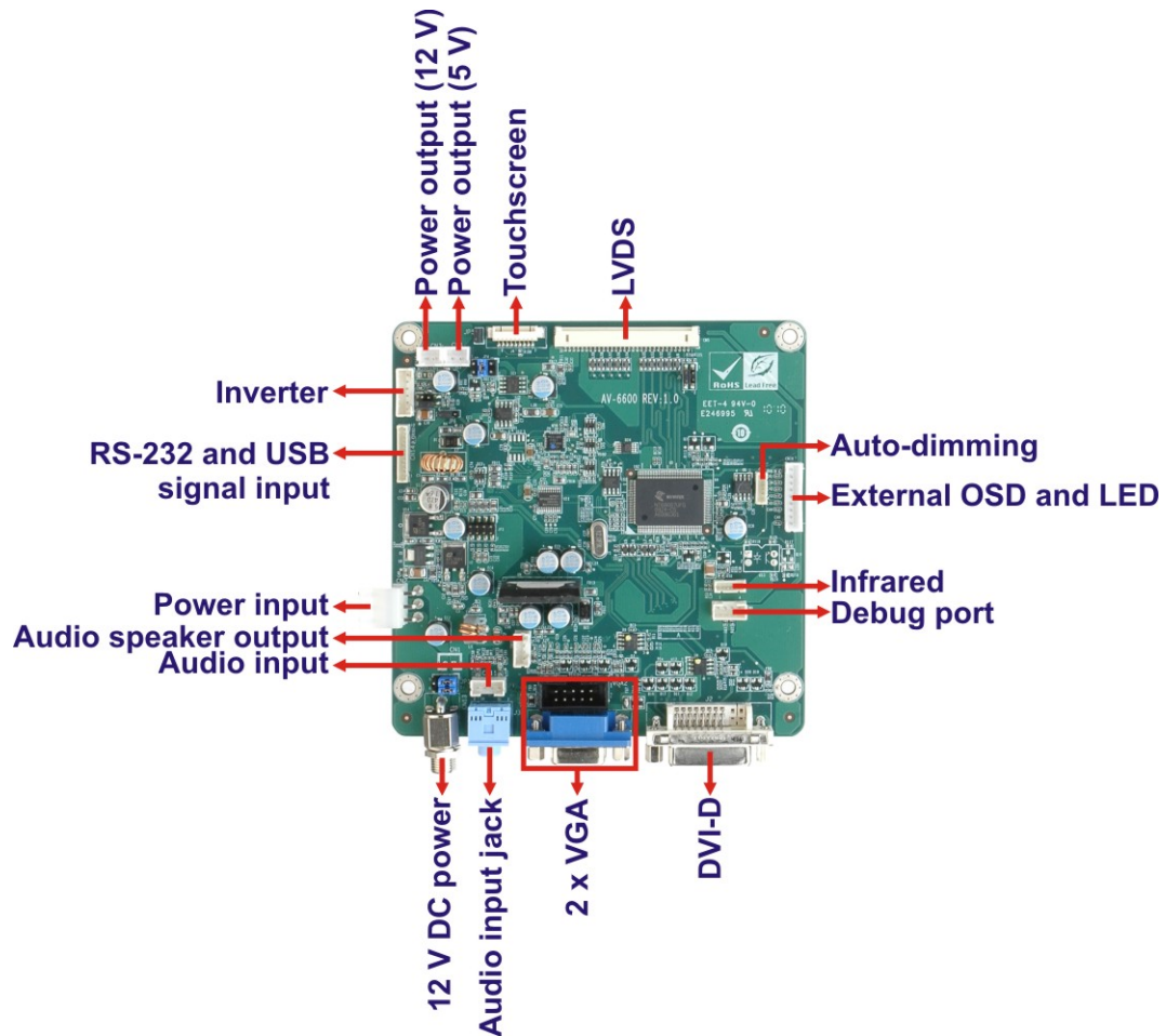
Figure 1-4: AV-6600 AD Board
