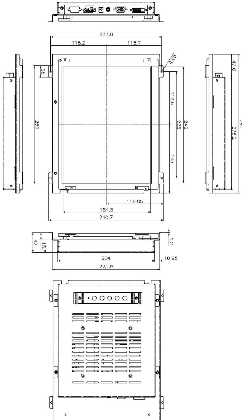
Figure 2-6: LCD-KIT121G/GX Physical Dimensions (millimeters)
