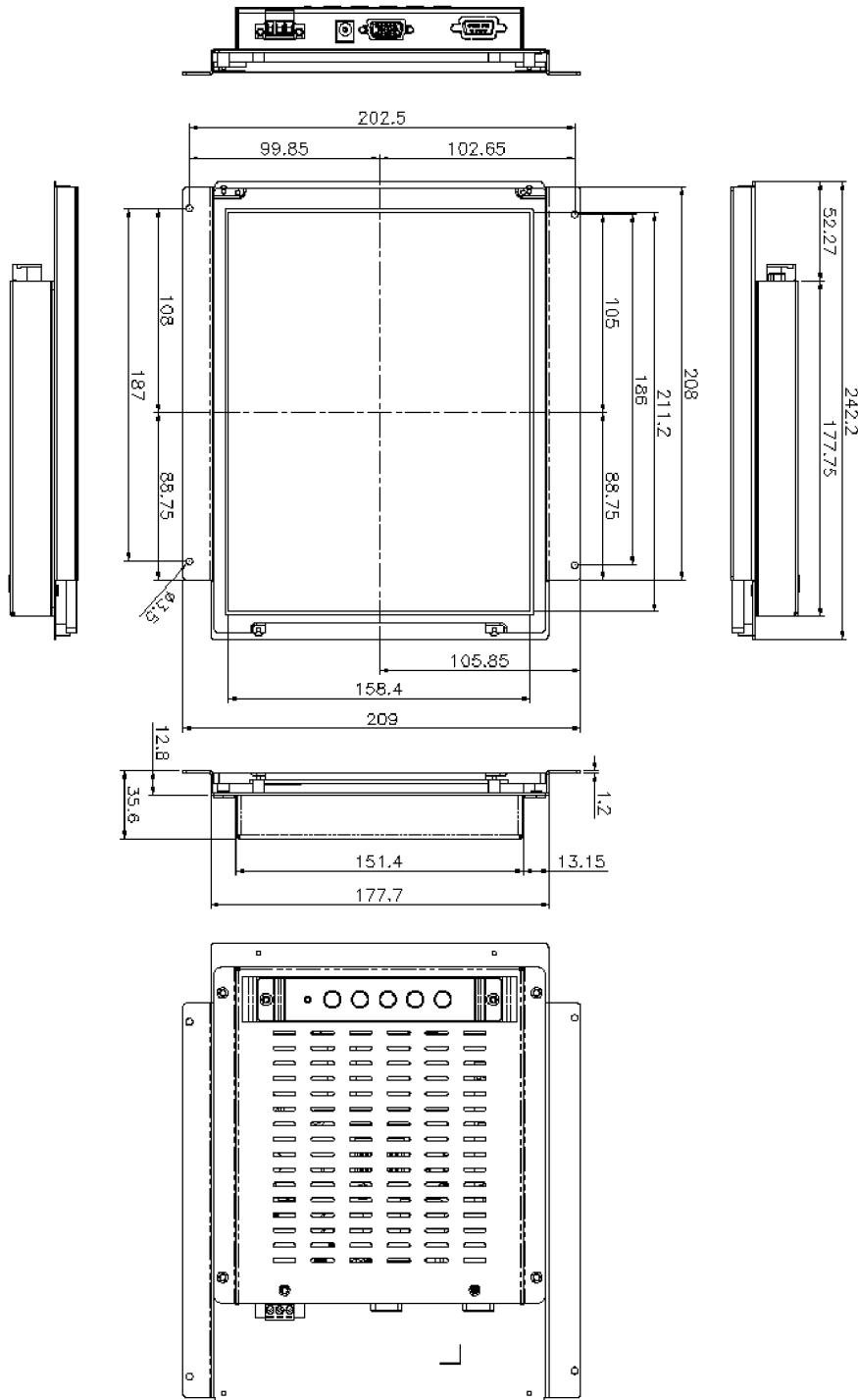
Figure 2-7: LCD-KIT104GH Physical Dimensions (millimeters)
