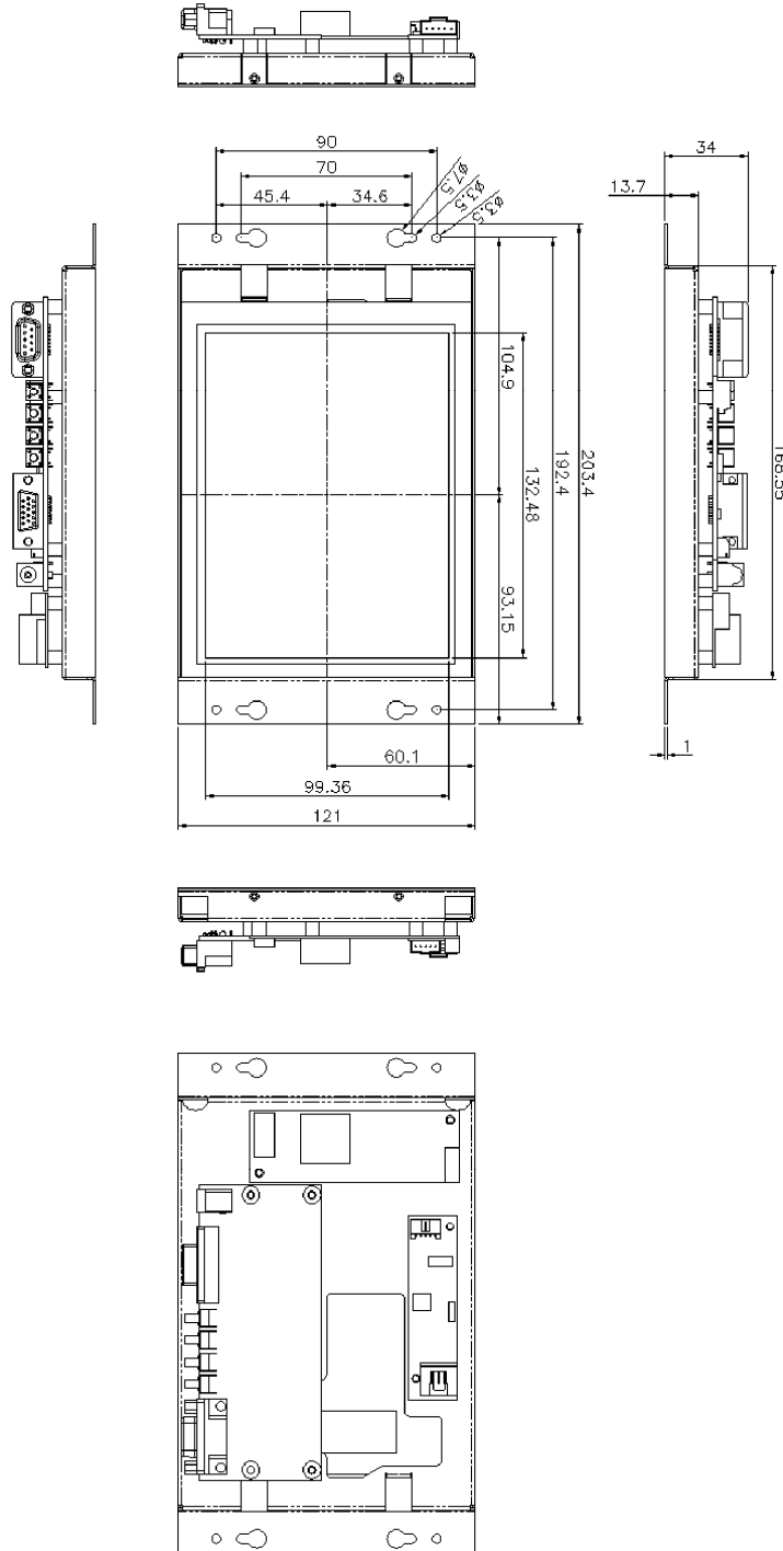
Figure 2-9: LCD-KIT65GH Physical Dimensions (millimeters)
