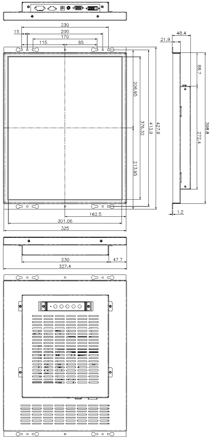
Figure 2-3: LCD-KIT190G Physical Dimensions (millimeters)
