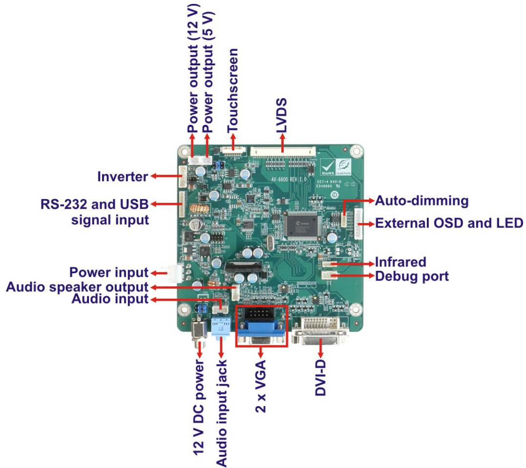
Figure 4-3: AV-6600 AD Board Overview
