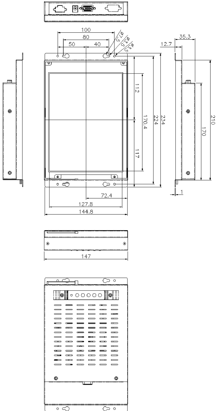
Figure 2-8: LCD-KIT84GH Physical Dimensions (millimeters)
