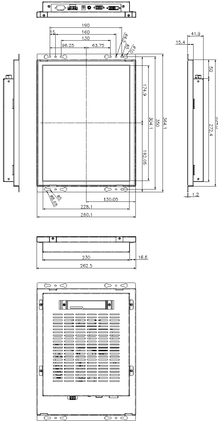
Figure 2-5: LCD-KIT150G Physical Dimensions (millimeters)
