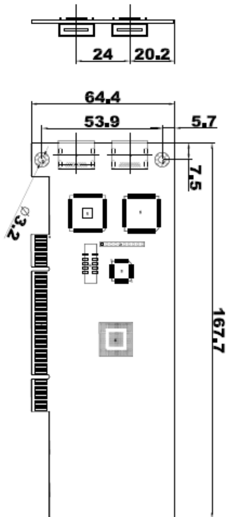
Figure 1-6: HDC-301 Dimensions (mm)
