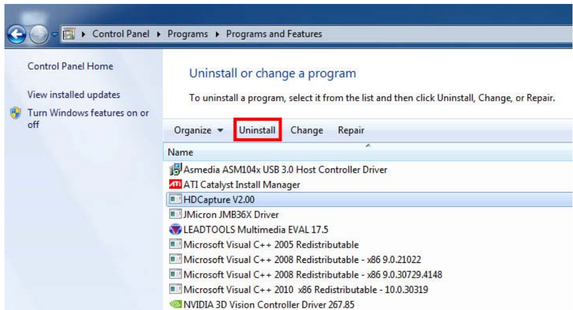
Figure 4-10: Uninstall HDCapture
