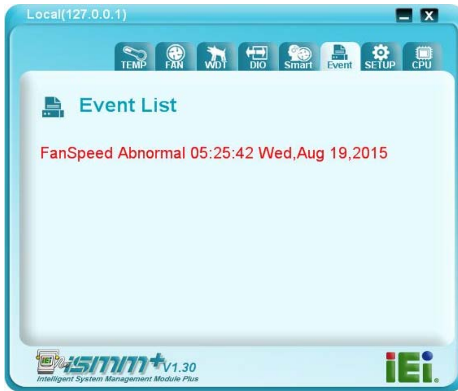
Figure 10: Event Page
