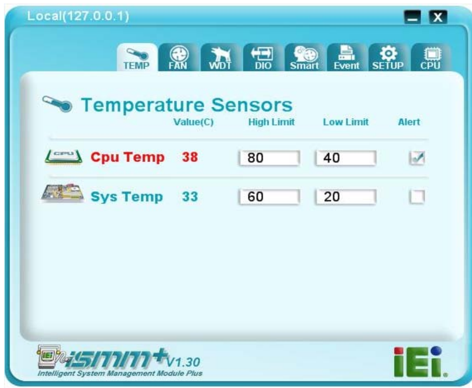
Figure 2: Temperature Page
